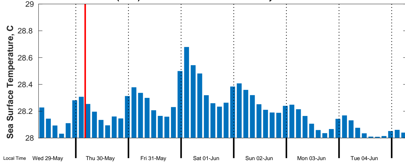
Sea Surface Temperature Forecast for CreOcean (Total) Block 6 EBS Suriname from 30-May-2024 00:00:00 to 06-Jun-2024 00:00:00
