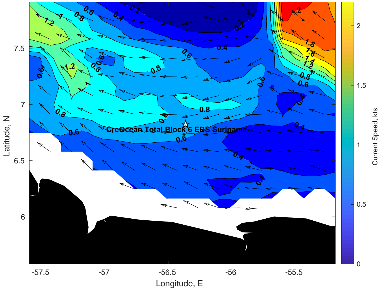
Surface Currents for CreOcean Total Block 6 EBS Suriname at 05-Aug-2024 00:00:00
