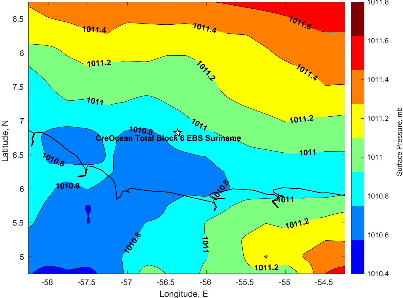
Surface Pressure (mb) for CreOcean Total Block 6 EBS Suriname at 06-Aug-2024 06:00:00
