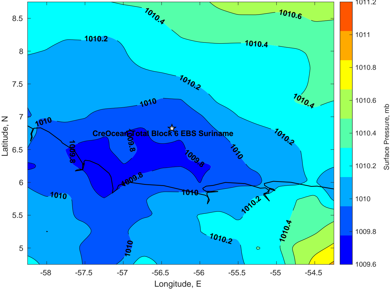
Surface Pressure (mb) for CreOcean Total Block 6 EBS Suriname at 07-Aug-2024 06:00:00
