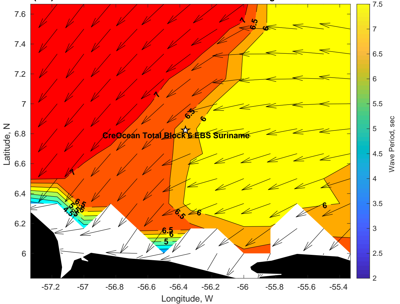
Wave Period (sec) for CreOcean Total Block 6 EBS Suriname at 05-Aug-2024 12:00:00
