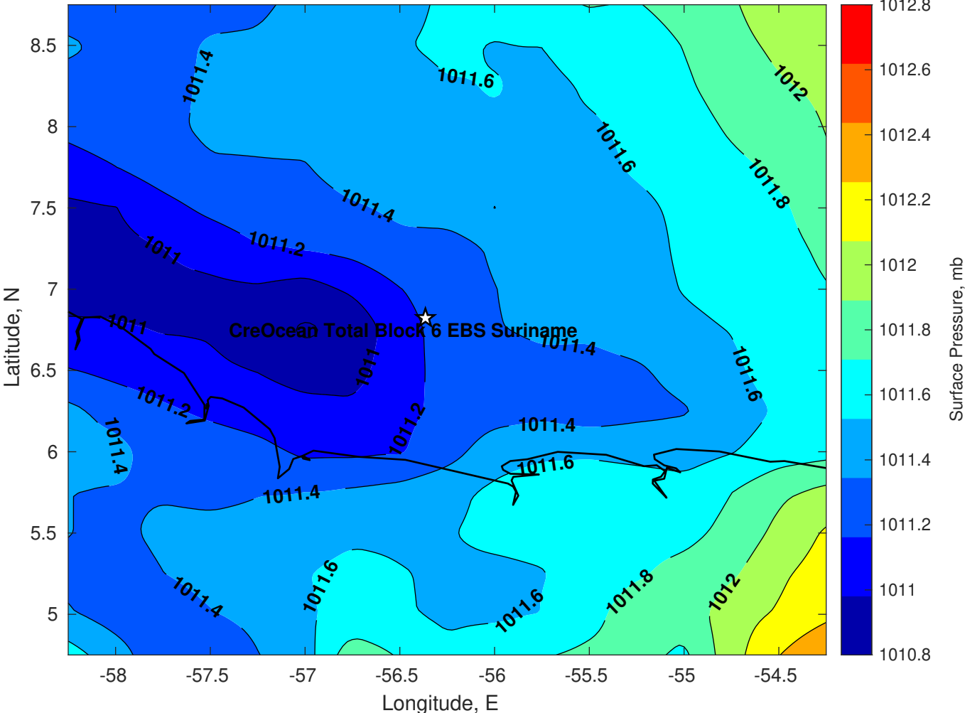
Surface Pressure (mb) for CreOcean Total Block 6 EBS Suriname at 05-Aug-2024 06:00:00
