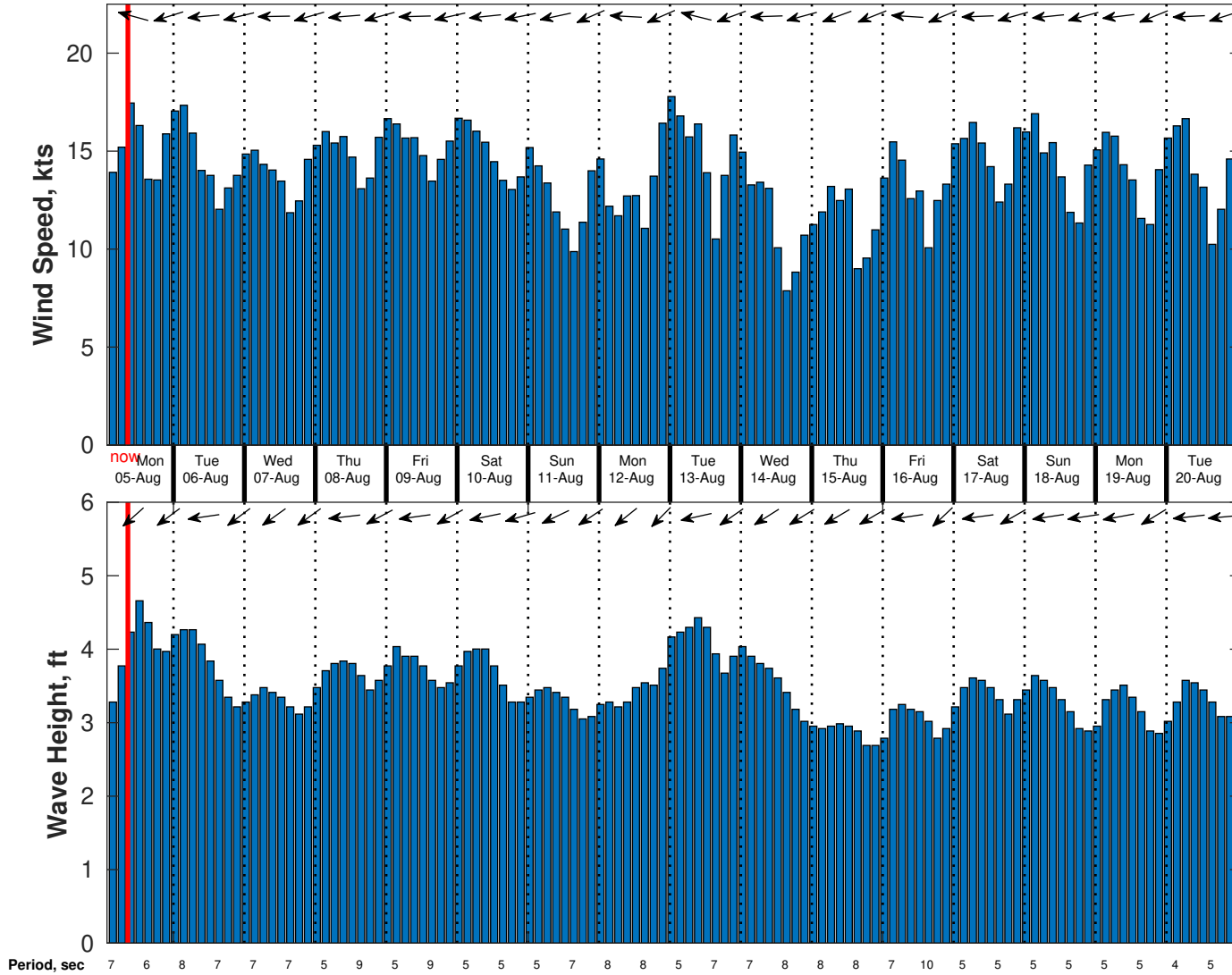
Wind & Wave Forecast for CreOcean Total Block 6 EBS Suriname from 05-Aug-2024 02:00:00 to 21-Aug-2024 02:00:00
