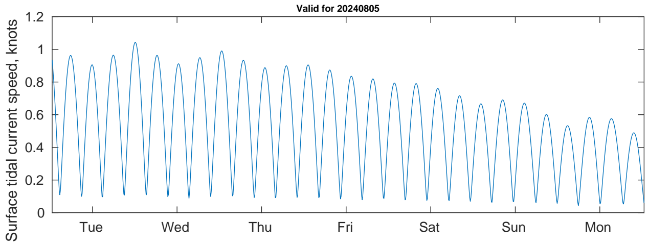
Tidal Currents and Heights for CreOcean Total Block 6 EBS Suriname at 20240805
