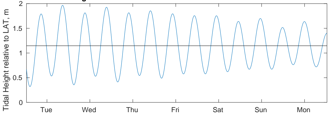
Tidal Currents and Heights for CreOcean Total Block 6 EBS Suriname at 20240805
