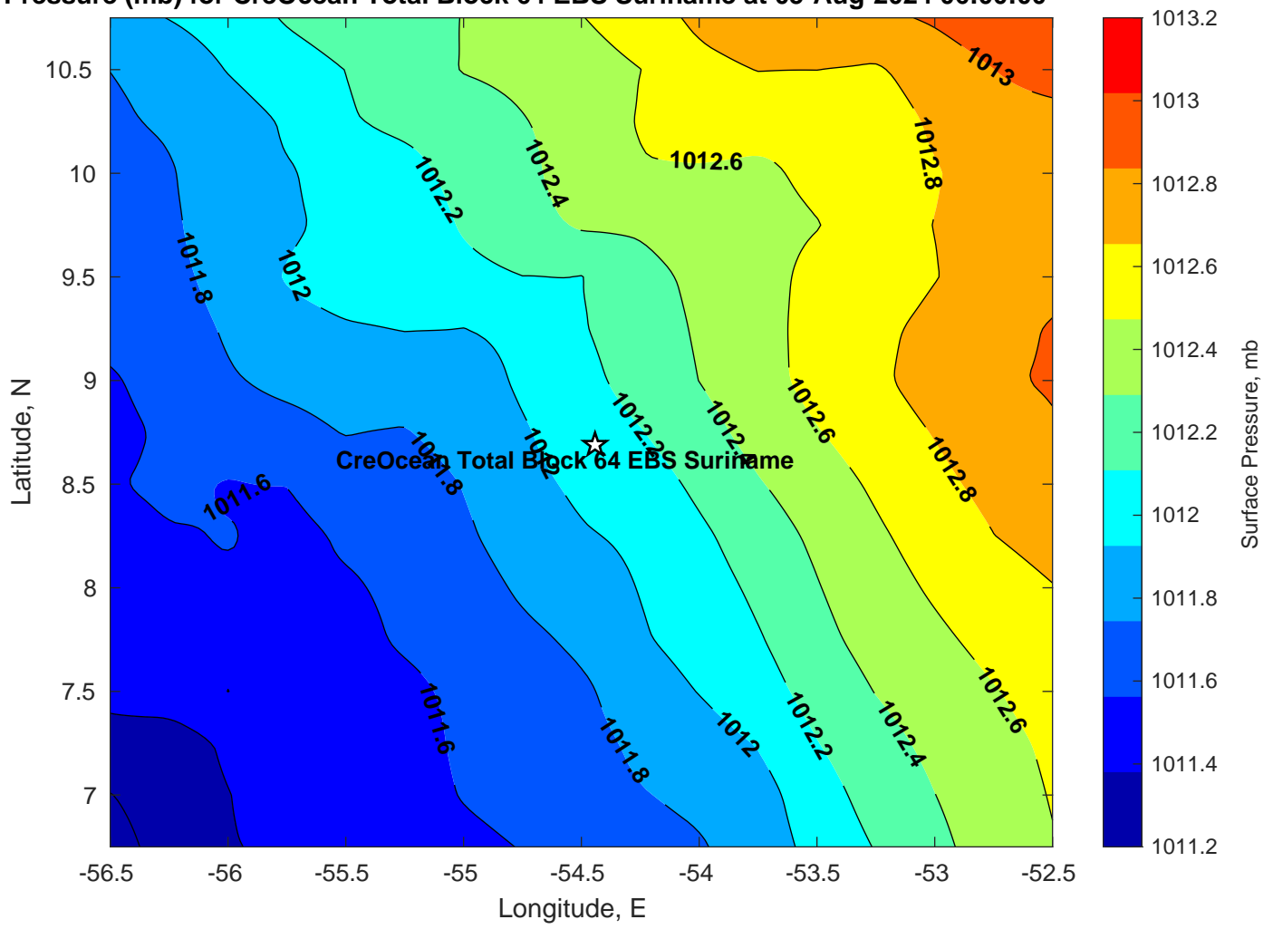
Surface Pressure (mb) for CreOcean Total Block 64 EBS Suriname at 05-Aug-2024 06:00:00
