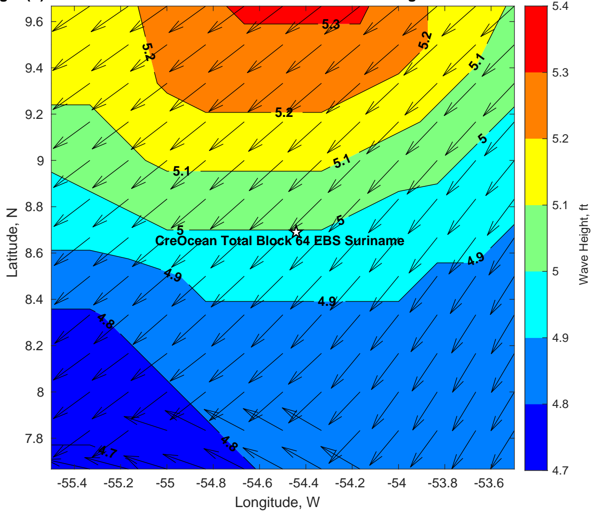
Wave Height (ft) for CreOcean Total Block 64 EBS Suriname at 05-Aug-2024 12:00:00
