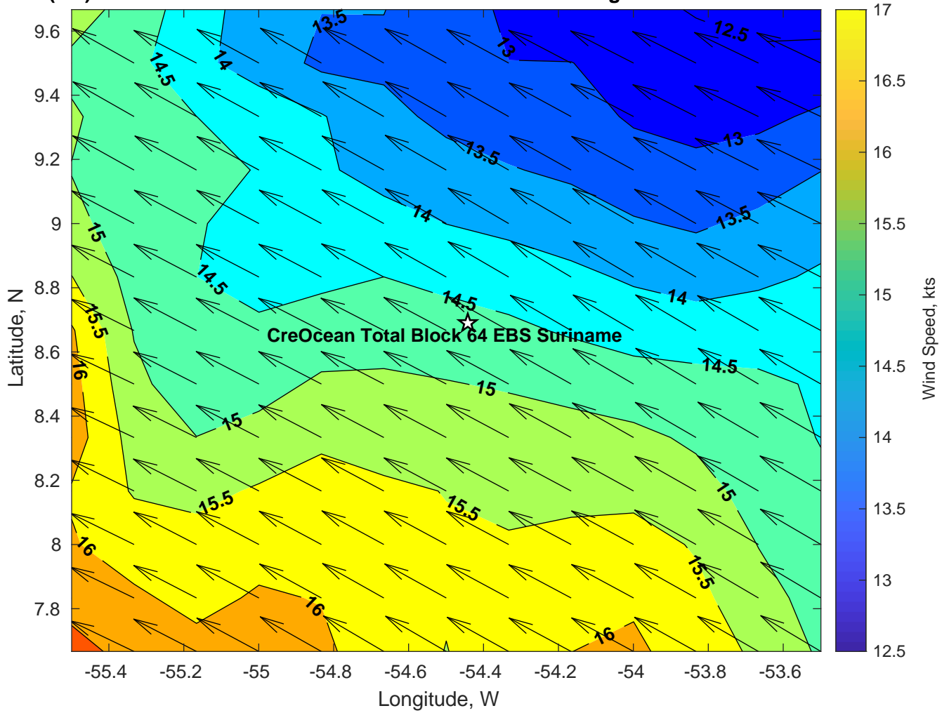
Winds (kts) for CreOcean Total Block 64 EBS Suriname at 05-Aug-2024 12:00:00
