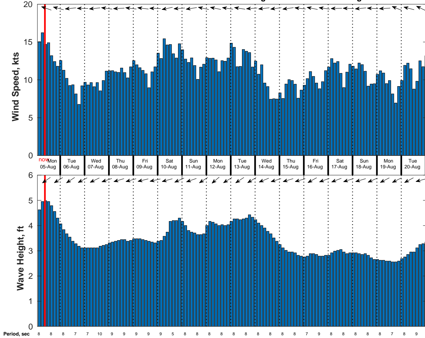
Wind & Wave Forecast for CreOcean Total Block 64 EBS Suriname from 05-Aug-2024 02:00:00 to 21-Aug-2024 02:00:00
