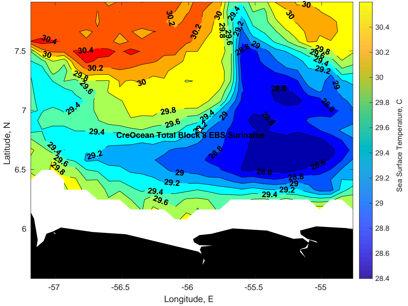
SST for CreOcean Total Block 8 EBS Suriname at 05-Aug-2024 00:00:00
