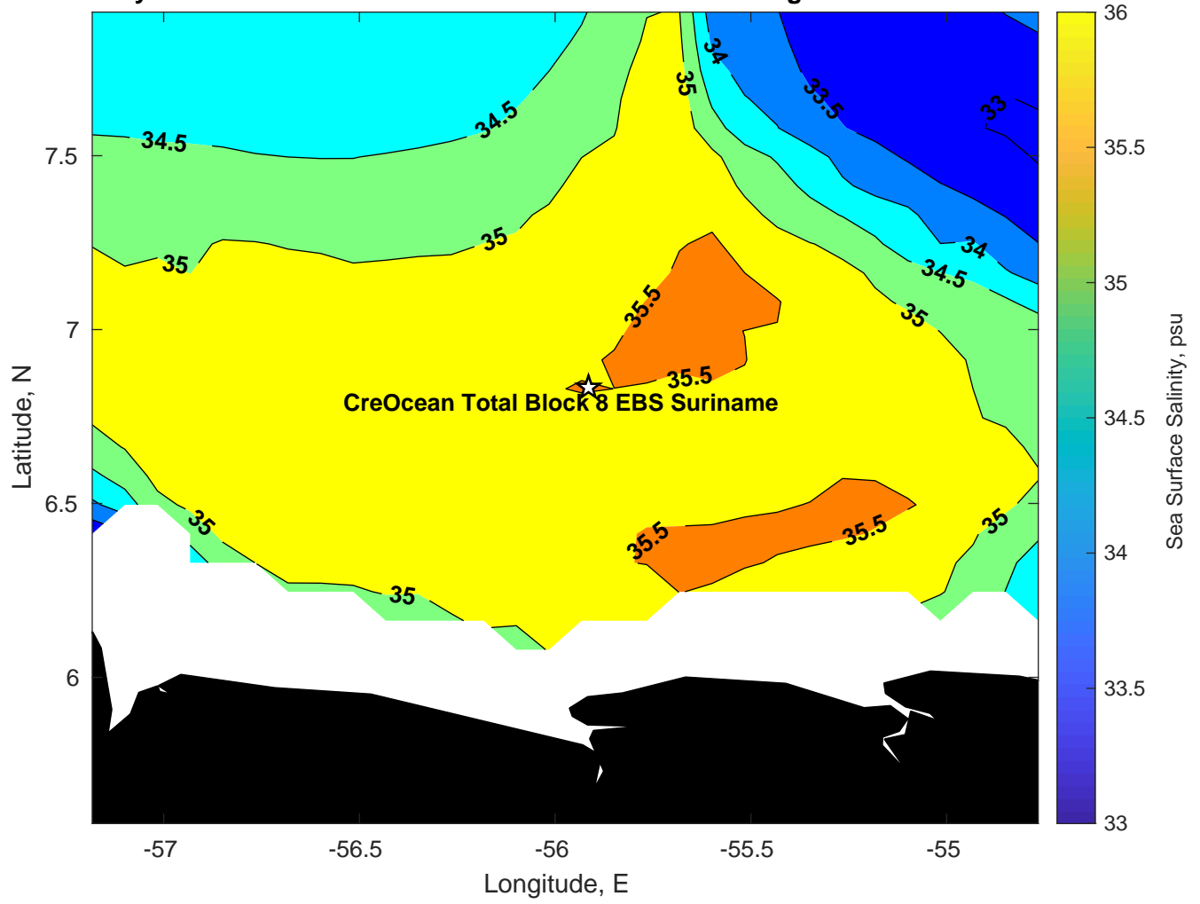
Surface Salinity for CreOcean Total Block 8 EBS Suriname at 05-Aug-2024 00:00:00
