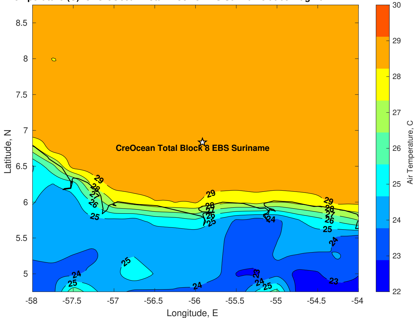
Air Temperature (C) for CreOcean Total Block 8 EBS Suriname at 05-Aug-2024
