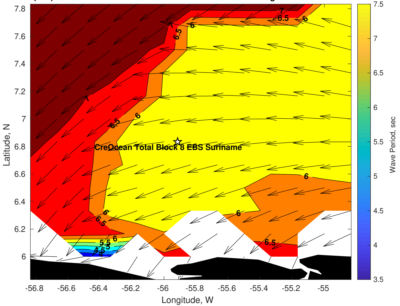
Wave Period (sec) for CreOcean Total Block 8 EBS Suriname at 05-Aug-2024 12:00:00
