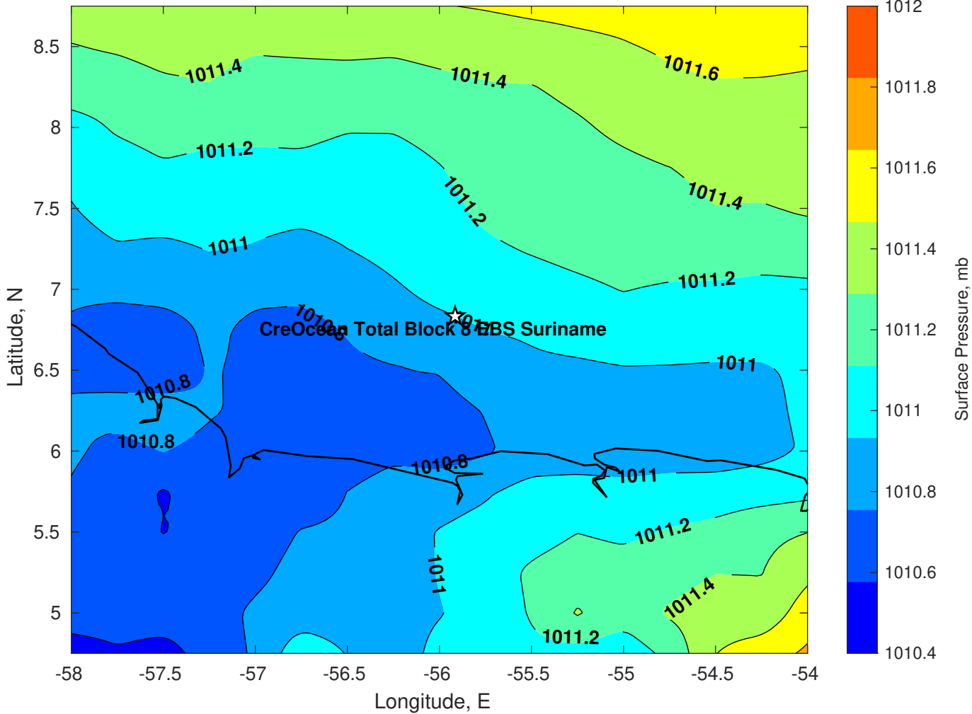
Surface Pressure (mb) for CreOcean Total Block 8 EBS Suriname at 06-Aug-2024 06:00:00
