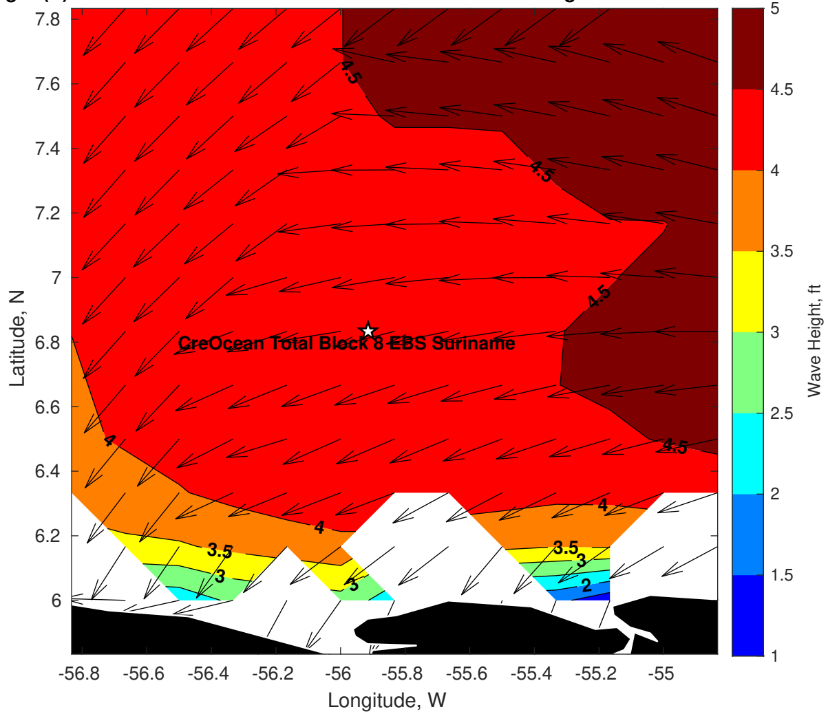
Wave Height (ft) for CreOcean Total Block 8 EBS Suriname at 05-Aug-2024 12:00:00
