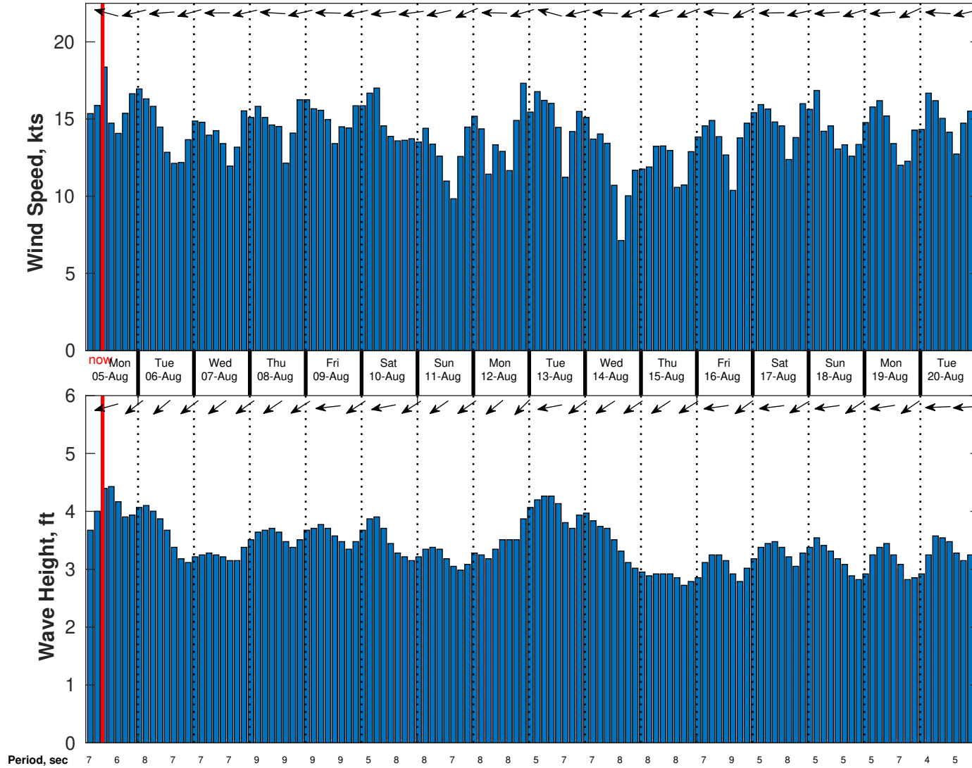
Wind & Wave Forecast for CreOcean Total Block 8 EBS Suriname from 05-Aug-2024 02:00:00 to 21-Aug-2024 02:00:00
