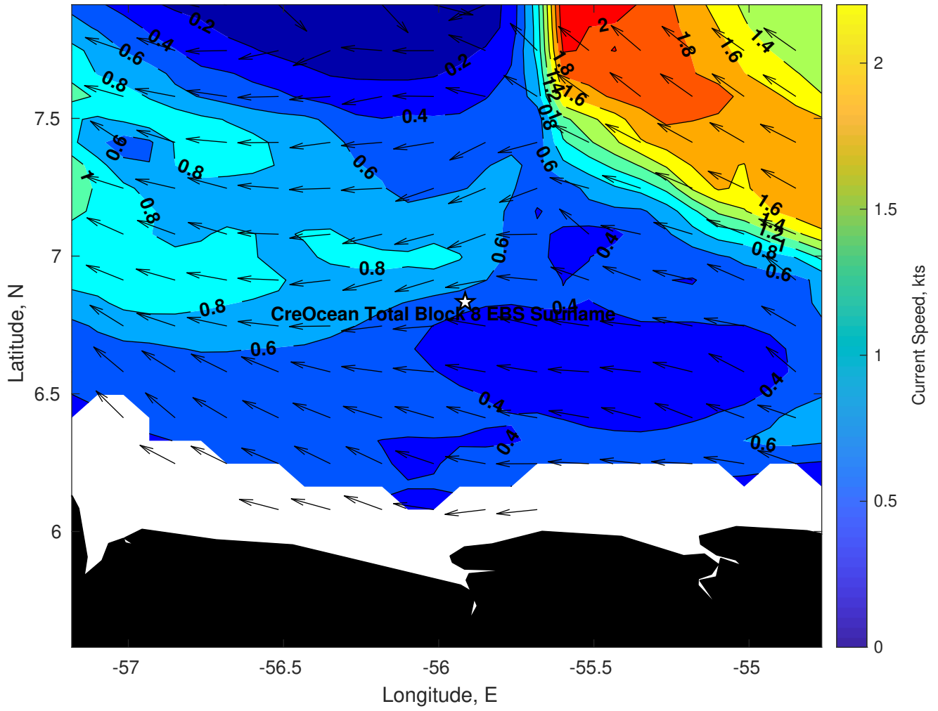
Surface Currents for CreOcean Total Block 8 EBS Suriname at 05-Aug-2024 00:00:00
