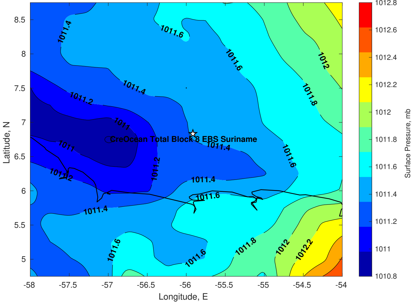
Surface Pressure (mb) for CreOcean Total Block 8 EBS Suriname at 05-Aug-2024 06:00:00
