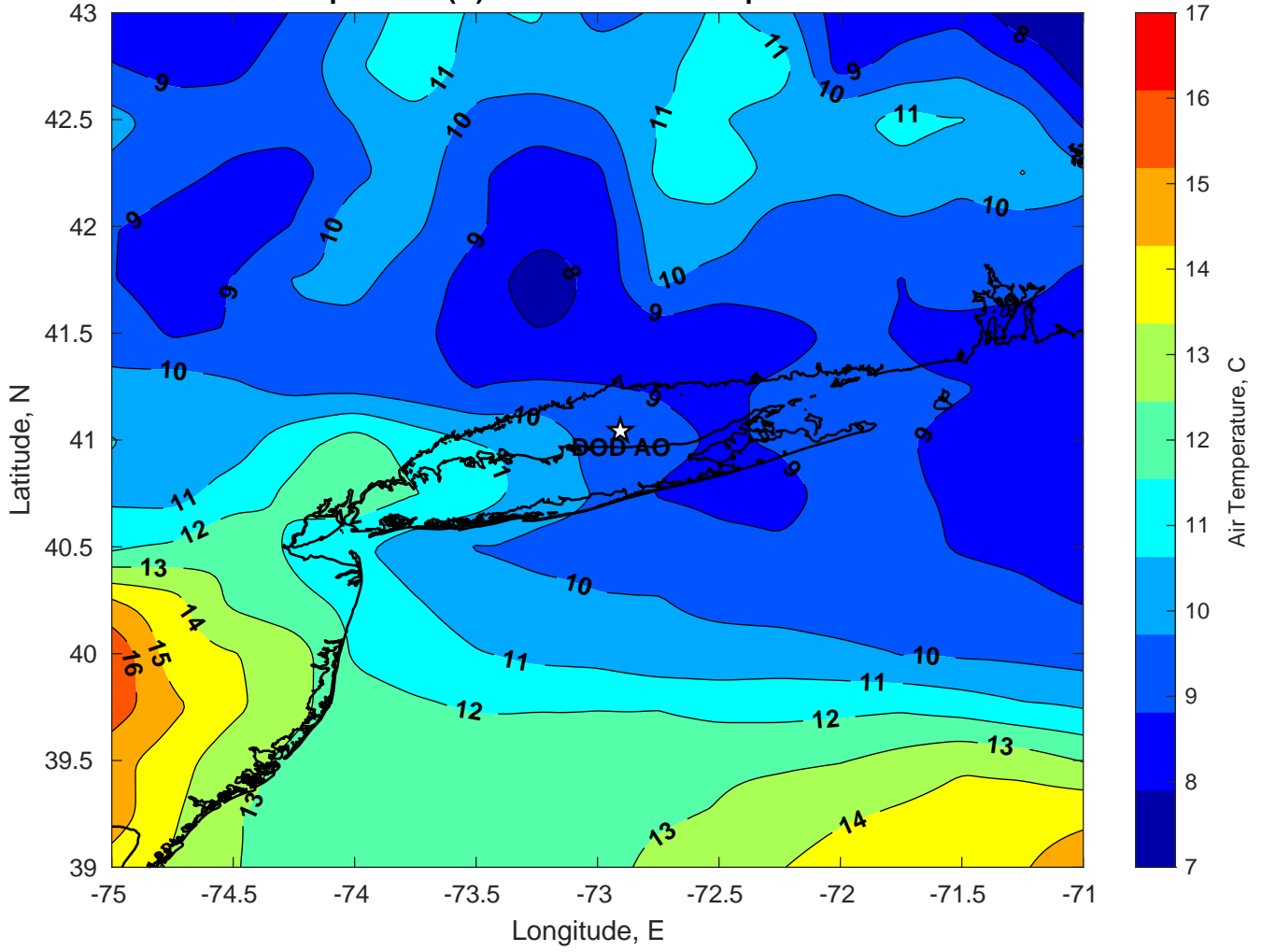
Air Temperature (C) for DOD AO at 17-Apr-2024
