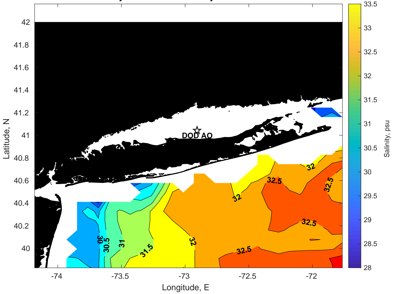
Surface Salinity for DOD AO at 03-May-2024 00:00:00
