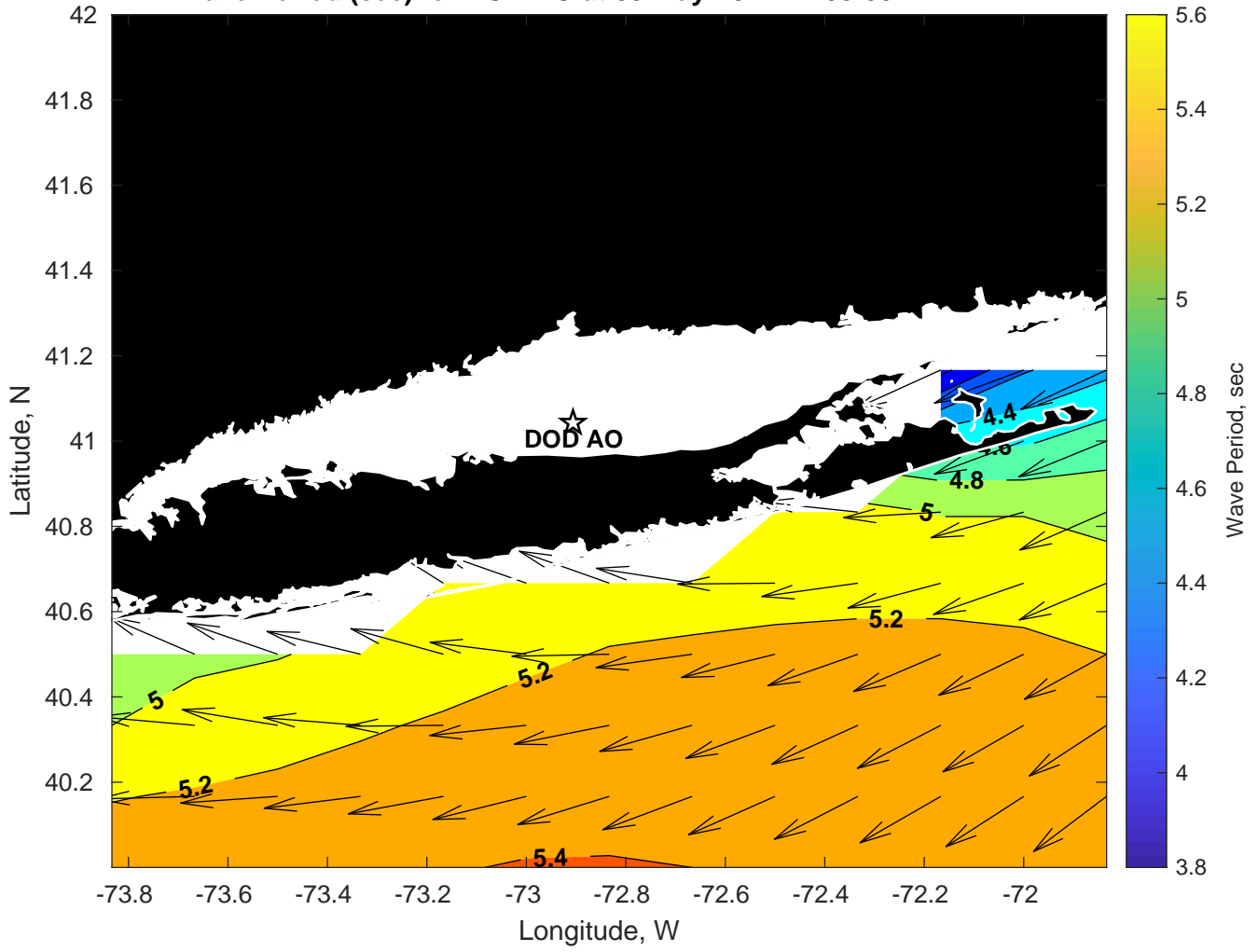
Wave Period (sec) for DOD AO at 03-May-2024 12:00:00
