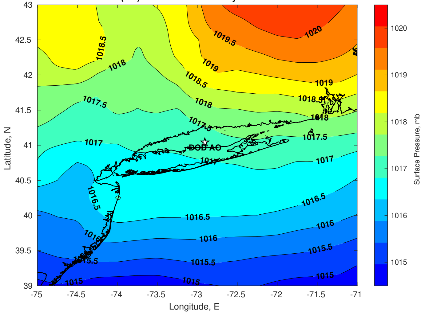
Surface Pressure (mb) for DOD AO at 03-May-2024 06:00:00
