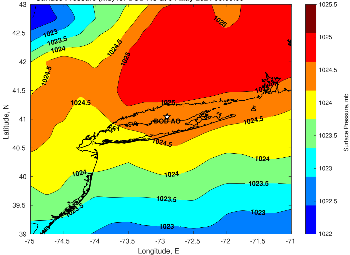
Surface Pressure (mb) for DOD AO at 04-May-2024 06:00:00
