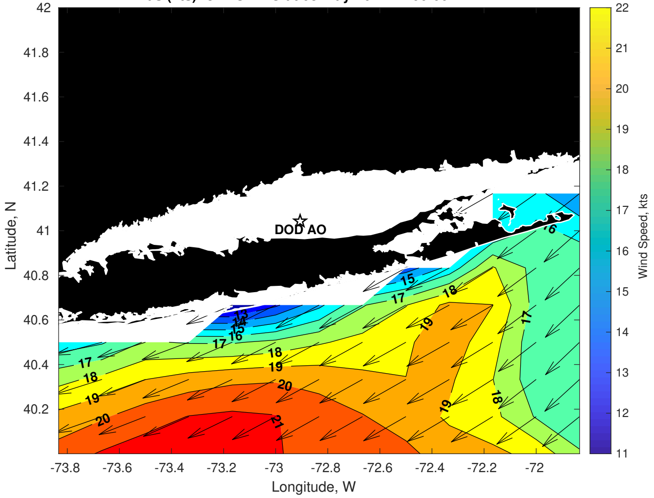
Winds (kts) for DOD AO at 03-May-2024 12:00:00
