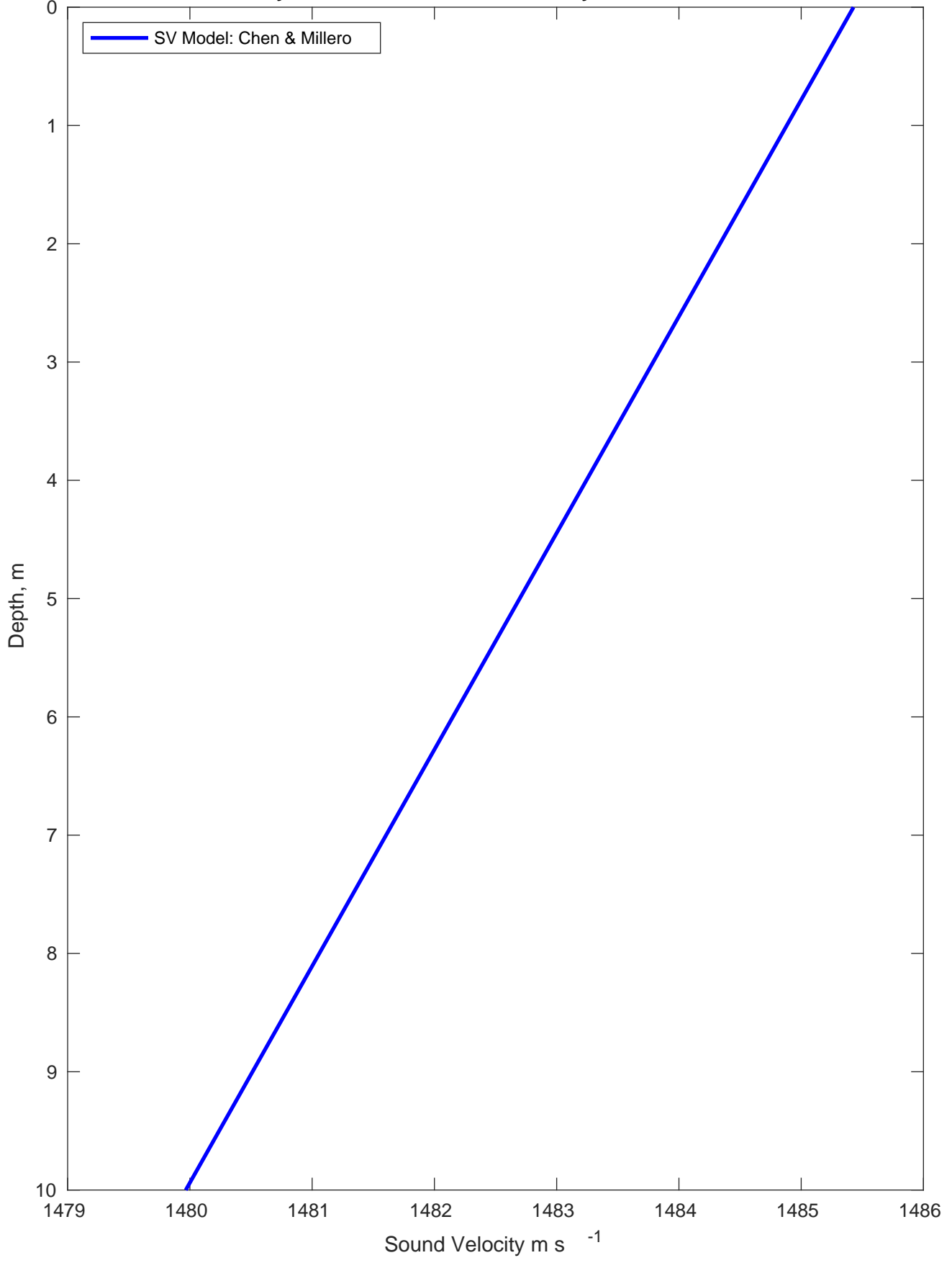
Sound Velocity Profile for DOD AO on 03-May-2024 00:00:00
