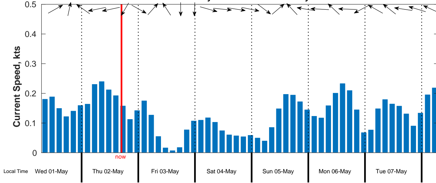
Current Forecast for DOD AO from 02-May-2024 00:00:00 to 09-May-2024 00:00:00
