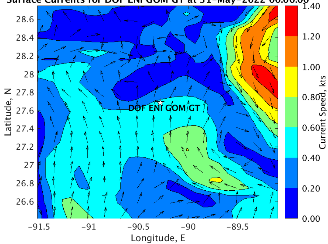
Surface Currents for DOF ENI GOM GT at 31-May-2022 00:00:00
