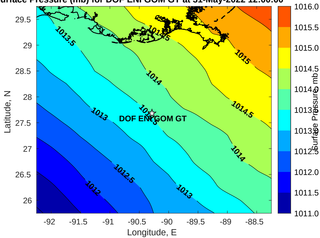
Surface Pressure (mb) for DOF ENI GOM GT at 31-May-2022 12:00:00
