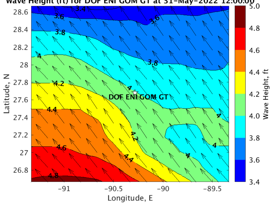
Wave Height (ft) for DOF ENI GOM GT at 31-May-2022 12:00:00
