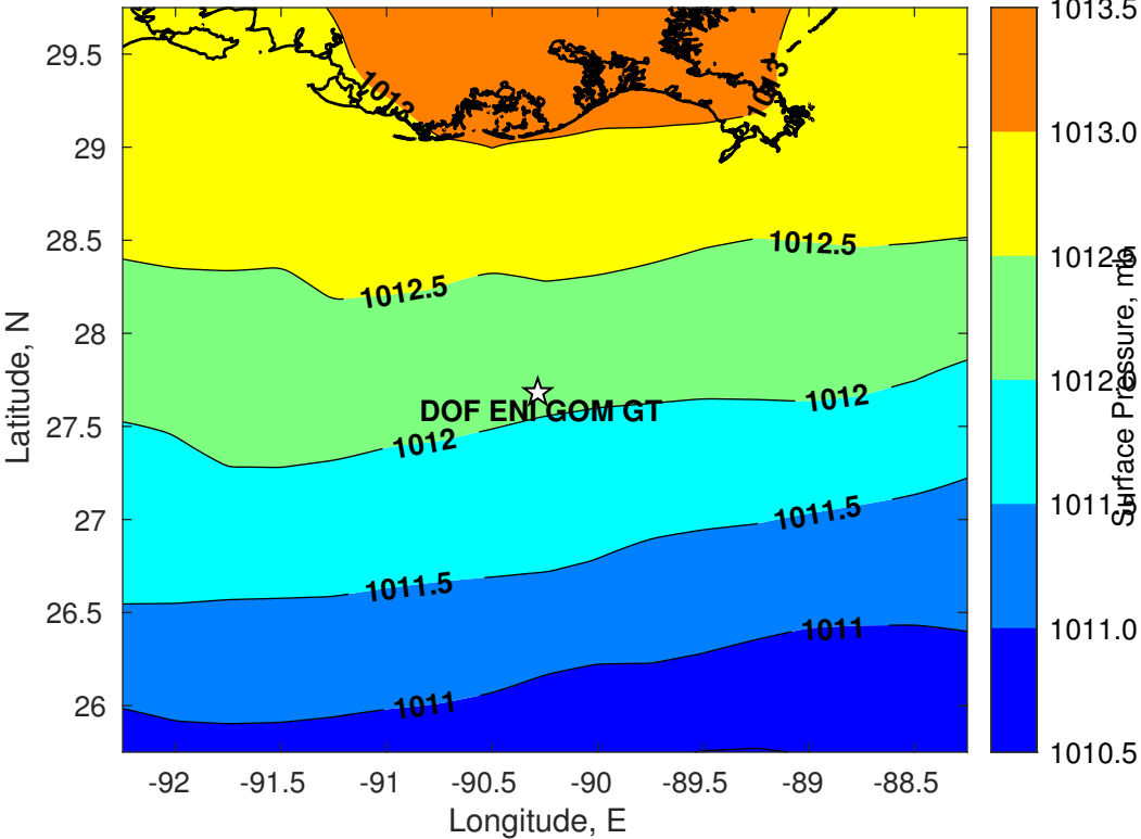
Surface Pressure (mb) for DOF ENI GOM GT at 02-Jun-2022 09:00:00
