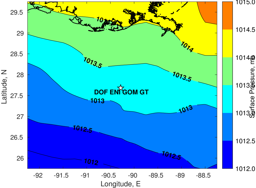
Surface Pressure (mb) for DOF ENI GOM GT at 01-Jun-2022 09:00:00
