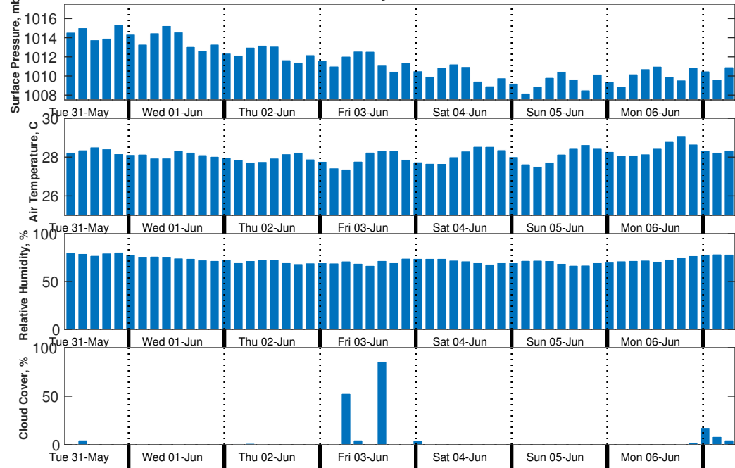
Met Forecast for DOF ENI GOM GT from 31-May-2022 12:00:00 to 07-Jun-2022 12:00:00
