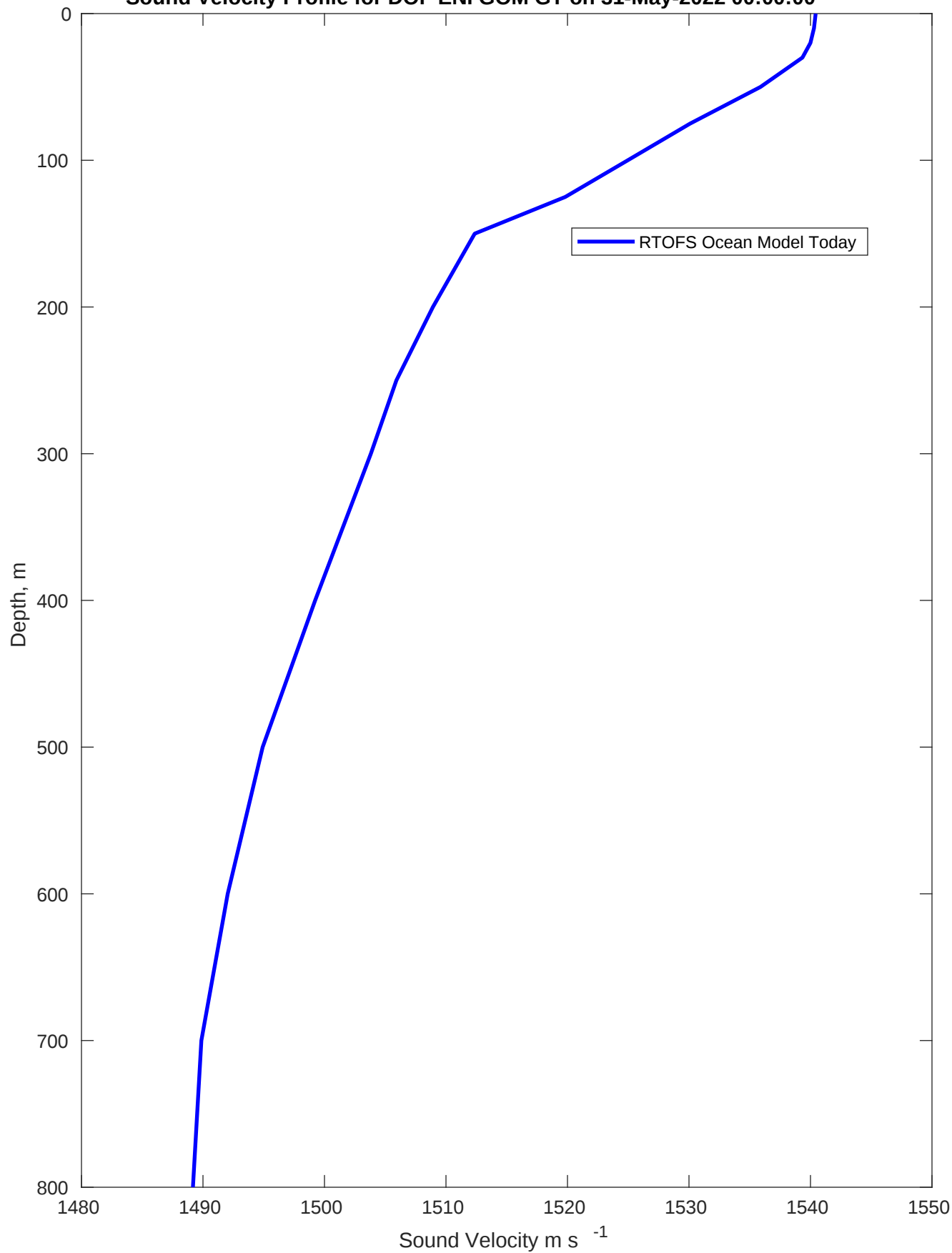
Sound Velocity Profile for DOF ENI GOM GT on 31-May-2022 00:00:00
