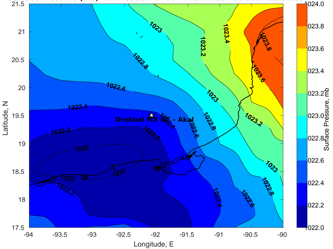
Surface Pressure (mb) for Drebbel MX GT - Akal at 21-Feb-2024 12:00:00
