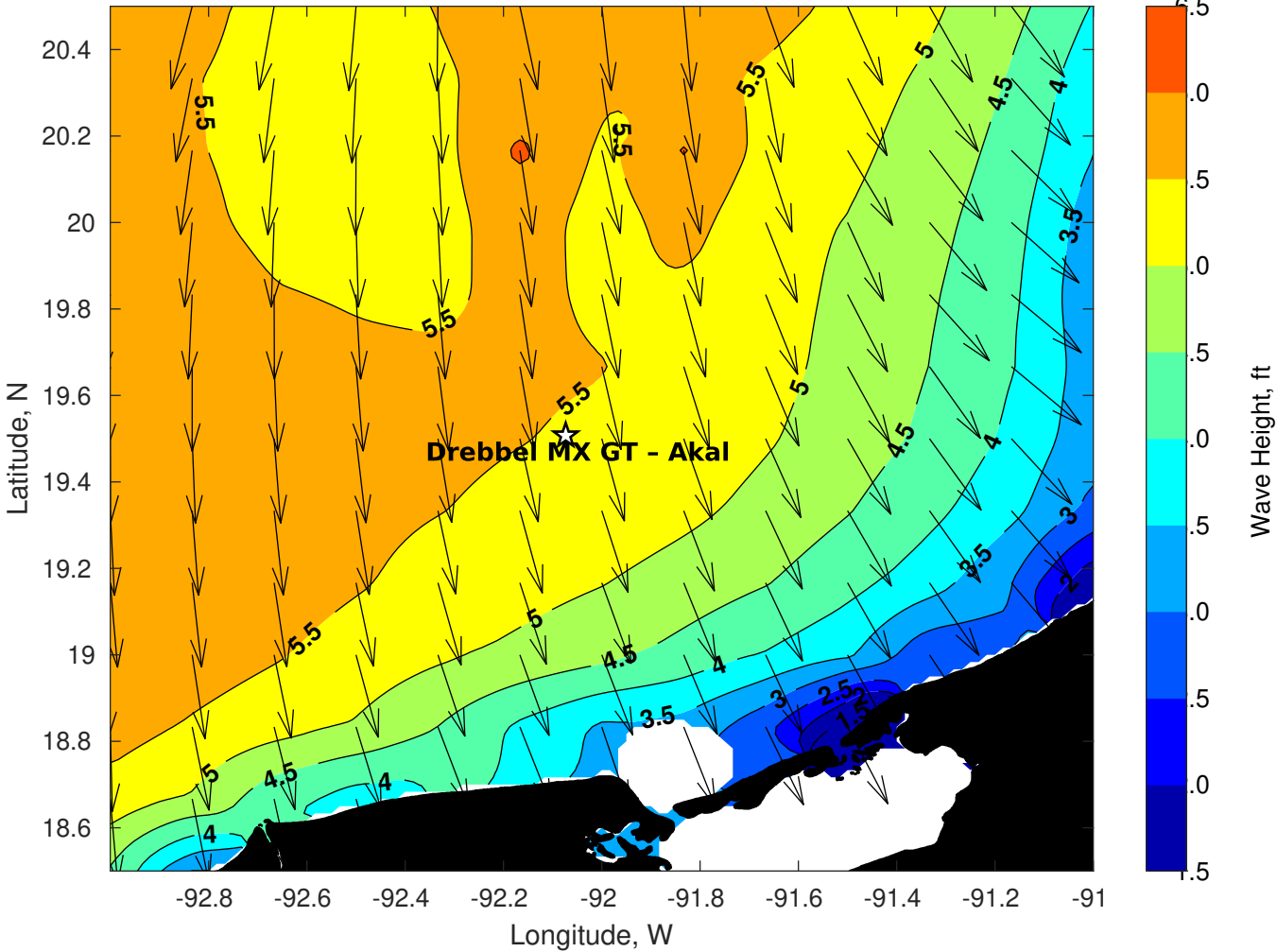
Wave Height (ft) for Drebbel MX GT - Akal at 19-Feb-2024 18:00:00
