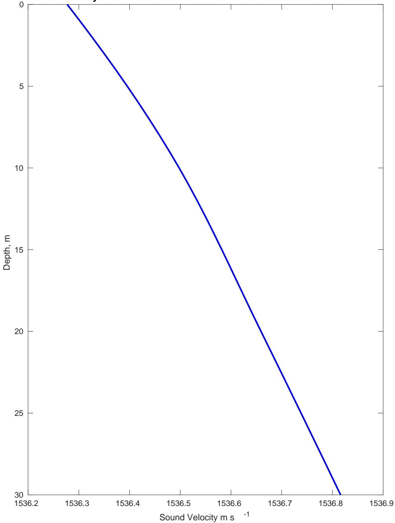
Sound Velocity Profile for Drebbel MX GT - Akal on 19-Feb-2024 00:00:00
