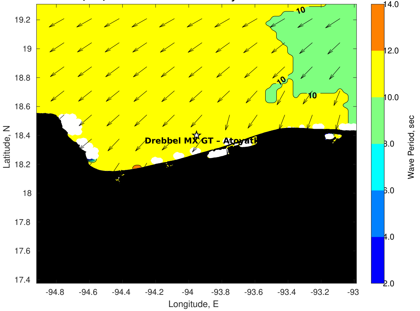
Wave Period (sec) for Drebbel MX GT - Atoyatl at 19-Feb-2024 18:00:00
