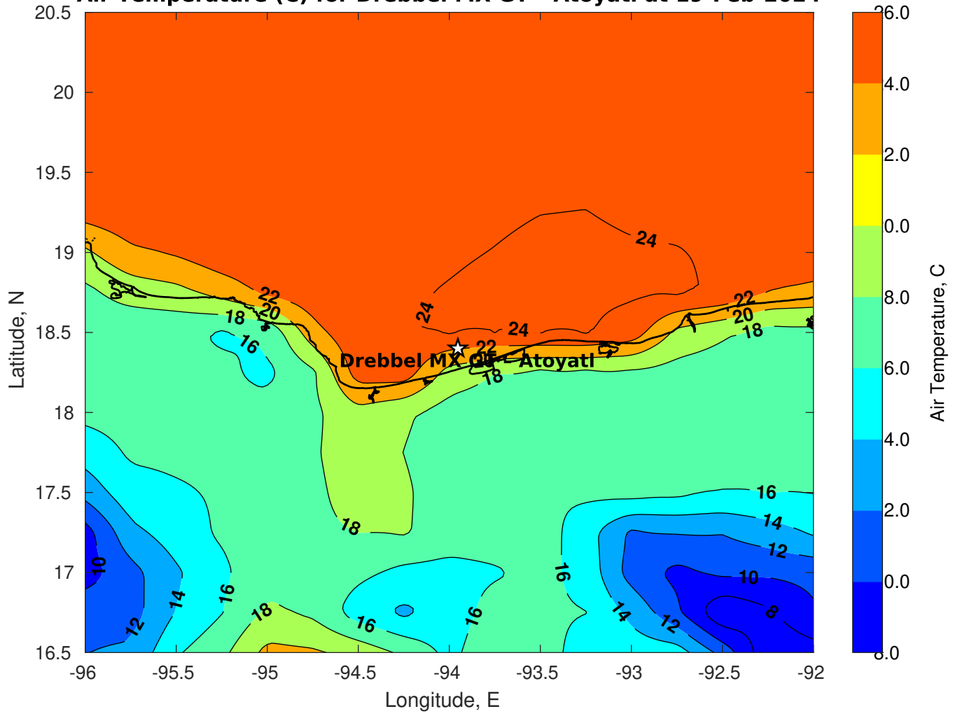
Air Temperature (C) for Drebbel MX GT - Atoyatl at 19-Feb-2024
