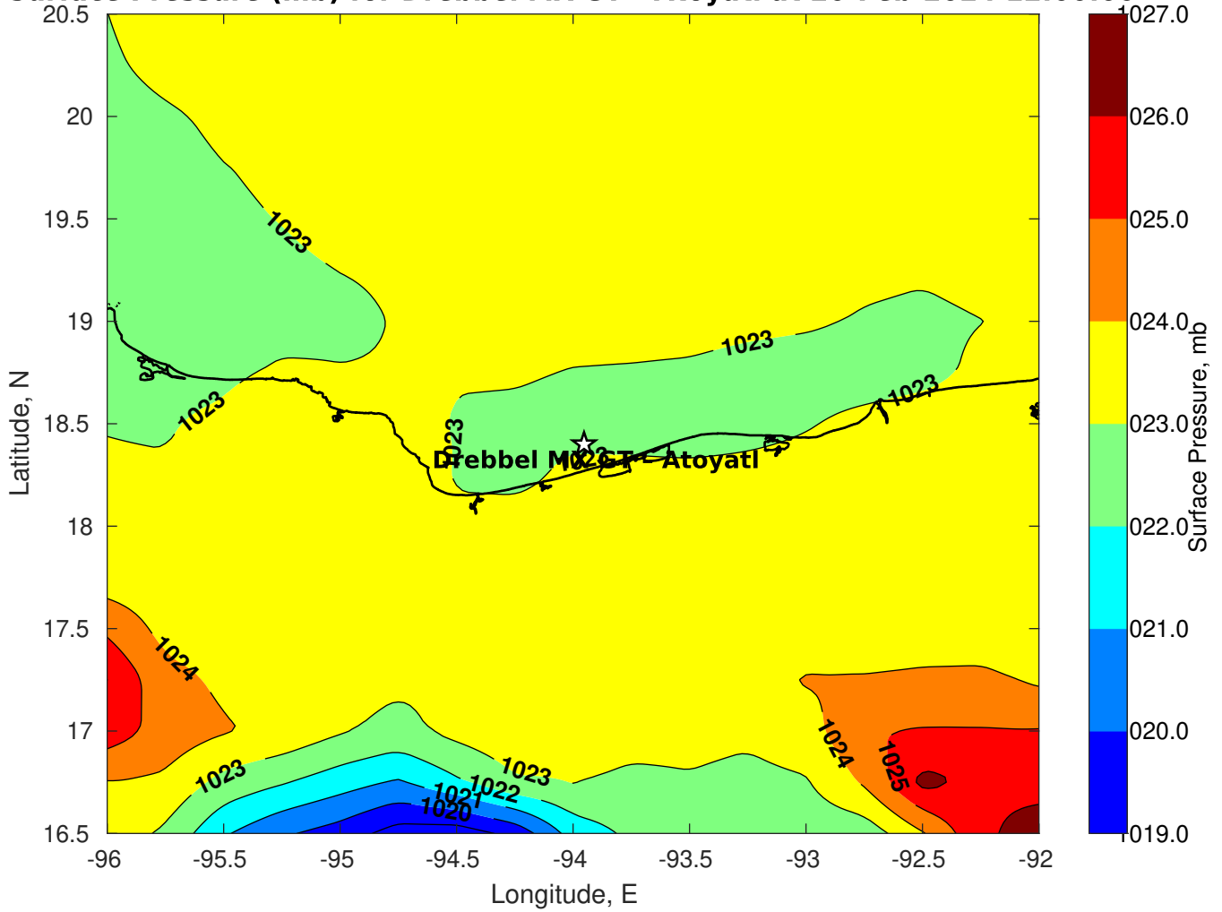
Surface Pressure (mb) for Drebbel MX GT - Atoyatl at 20-Feb-2024 12:00:00
