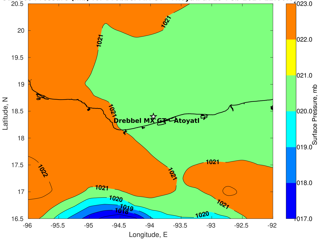
Surface Pressure (mb) for Drebbel MX GT - Atoyatl at 19-Feb-2024 12:00:00
