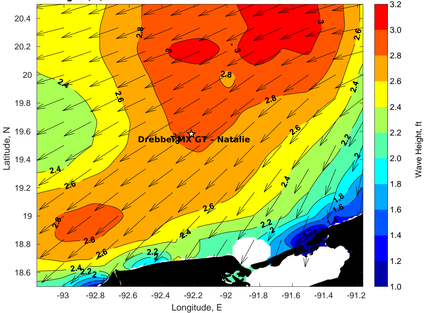
Wave Height (ft) for Drebbel MX GT - Natalie at 11-Mar-2023 12:00:00
