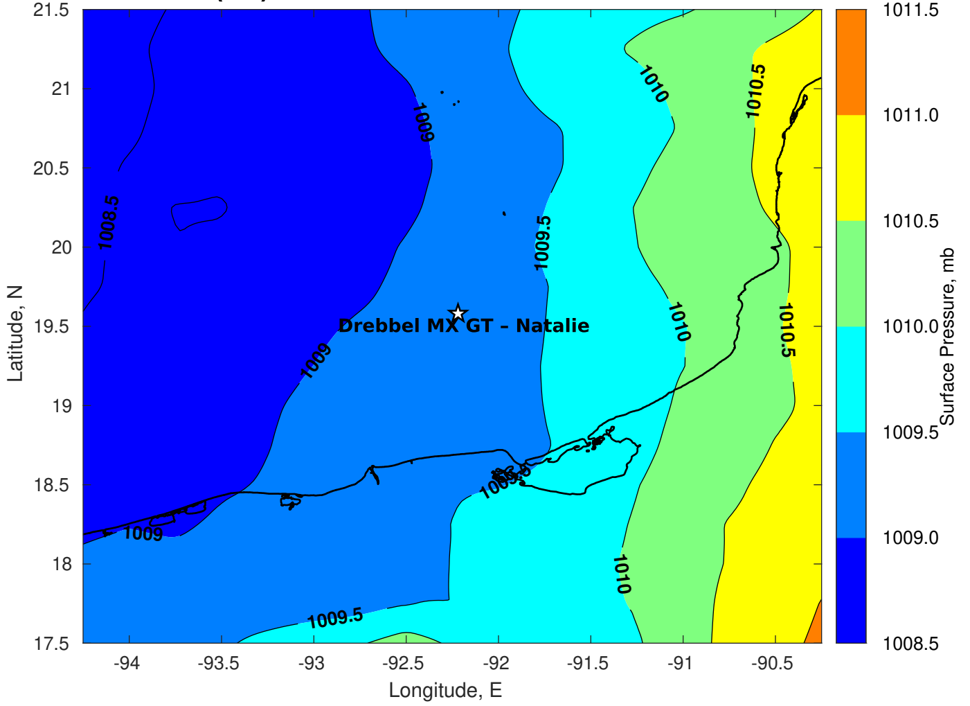
Surface Pressure (mb) for Drebbel MX GT - Natalie at 12-Mar-2023 12:00:00
