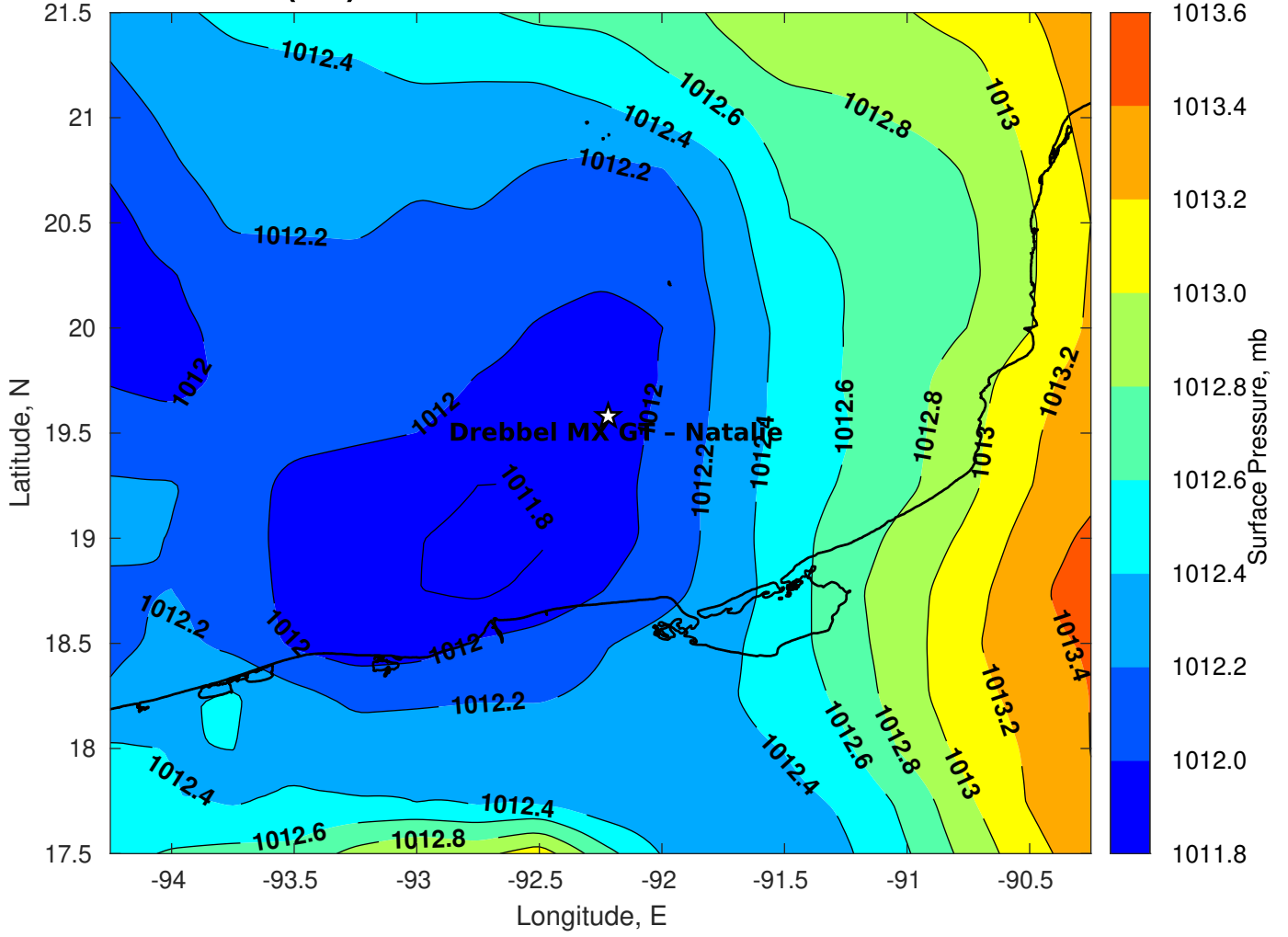
Surface Pressure (mb) for Drebhel MX GT - Natalie at 11-Mar-2023 12:00:00
