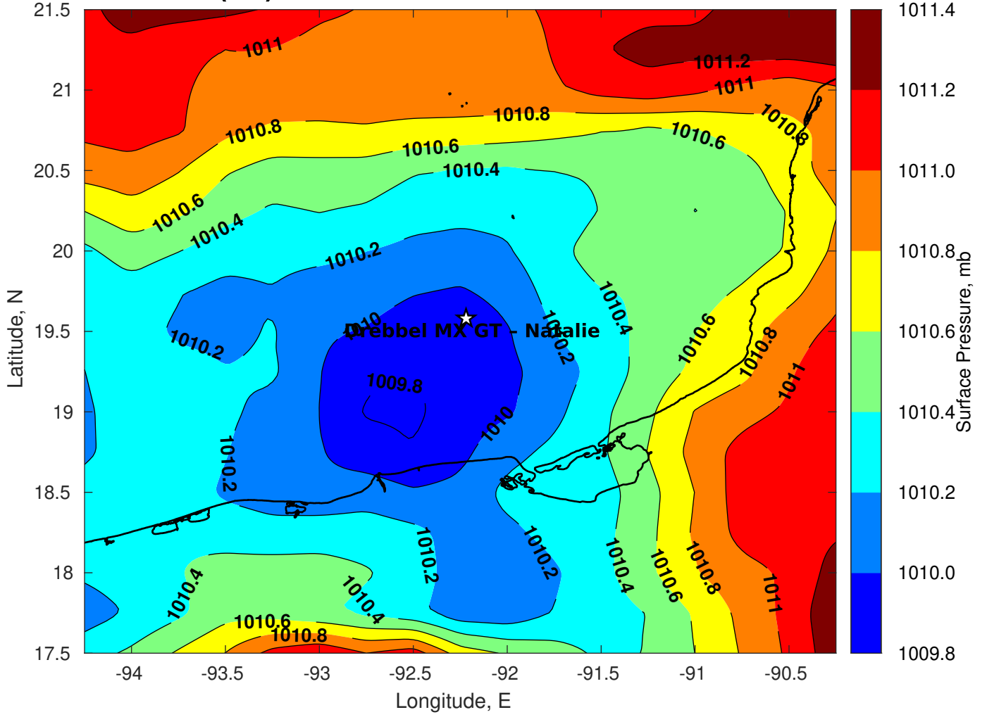
Surface Pressure (mb) for Drebberl MX GT - Natalie at 13-Mar-2023 12:00:00
