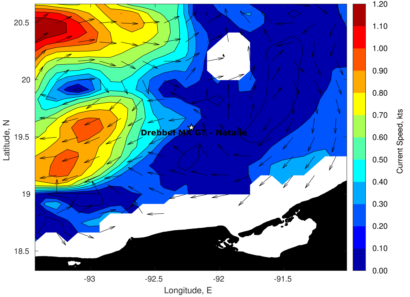
Surface Currents for Drebbel MX GT - Natalie at 11-Mar-2023 00:00:00
