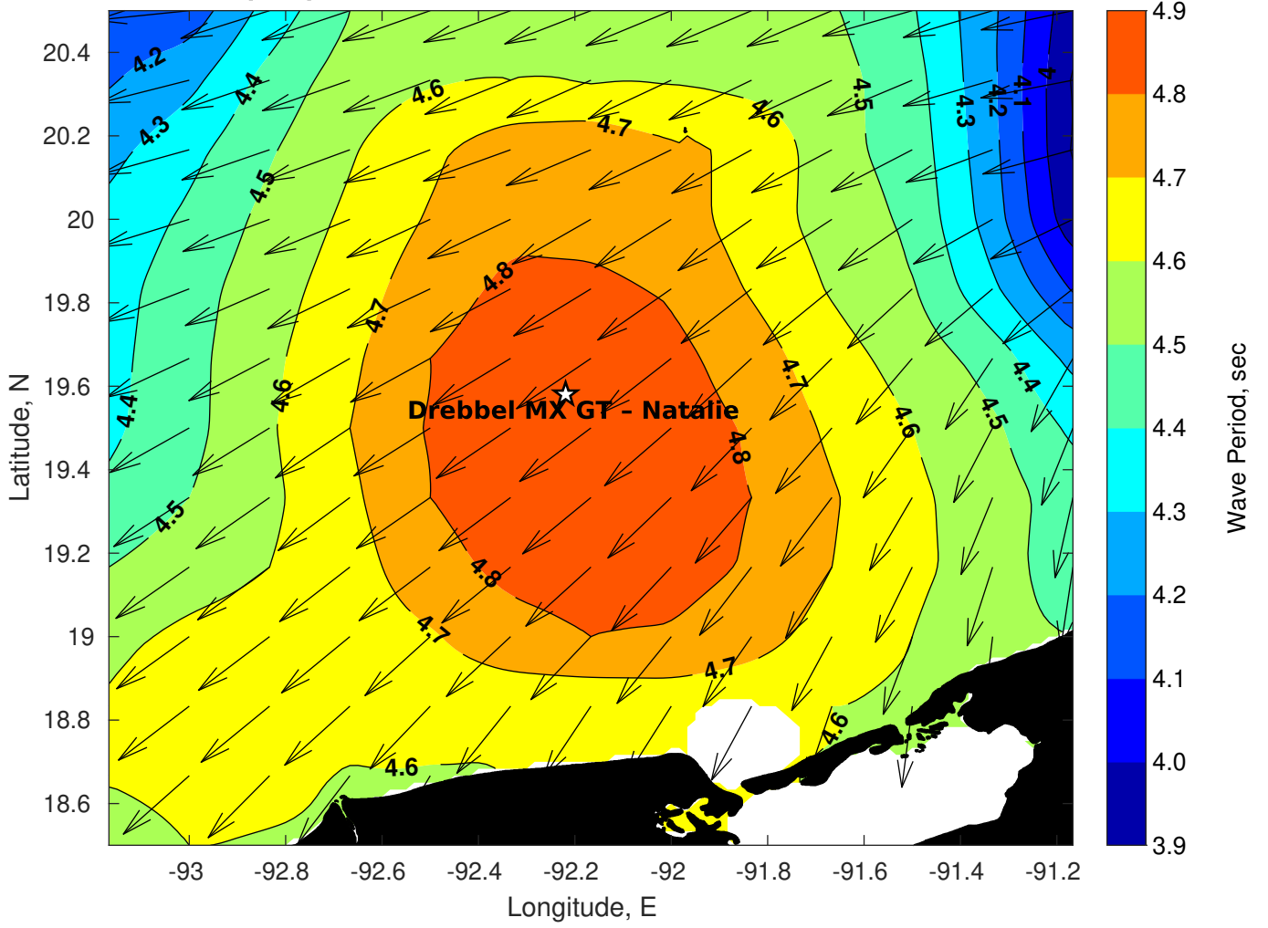
Wave Period (sec) for Drebbel MX GT - Natalie at 11-Mar-2023 12:00:00
