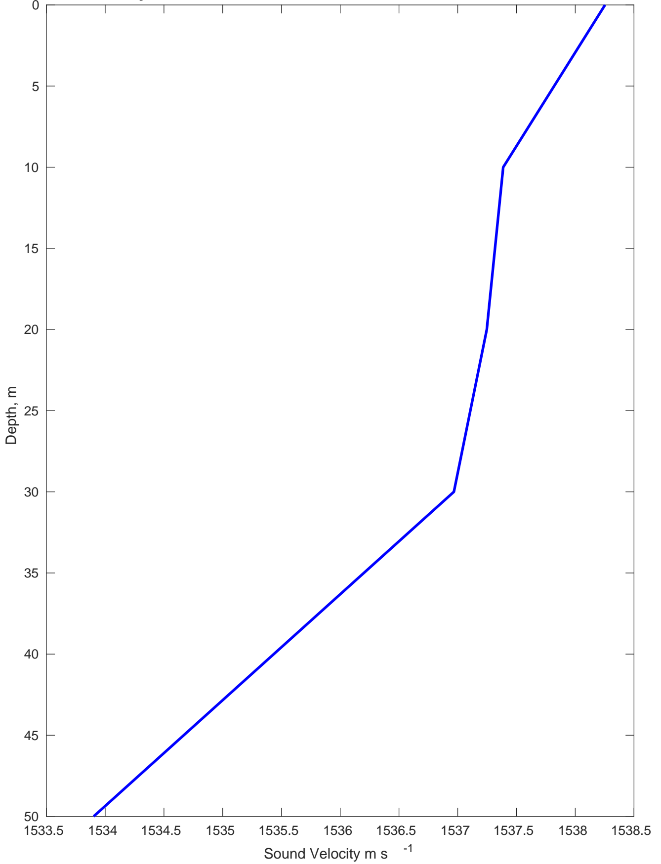
Sound Velocity Profile for Drebbel MX GT - Natalie on 11-Mar-2023 00:00:00
