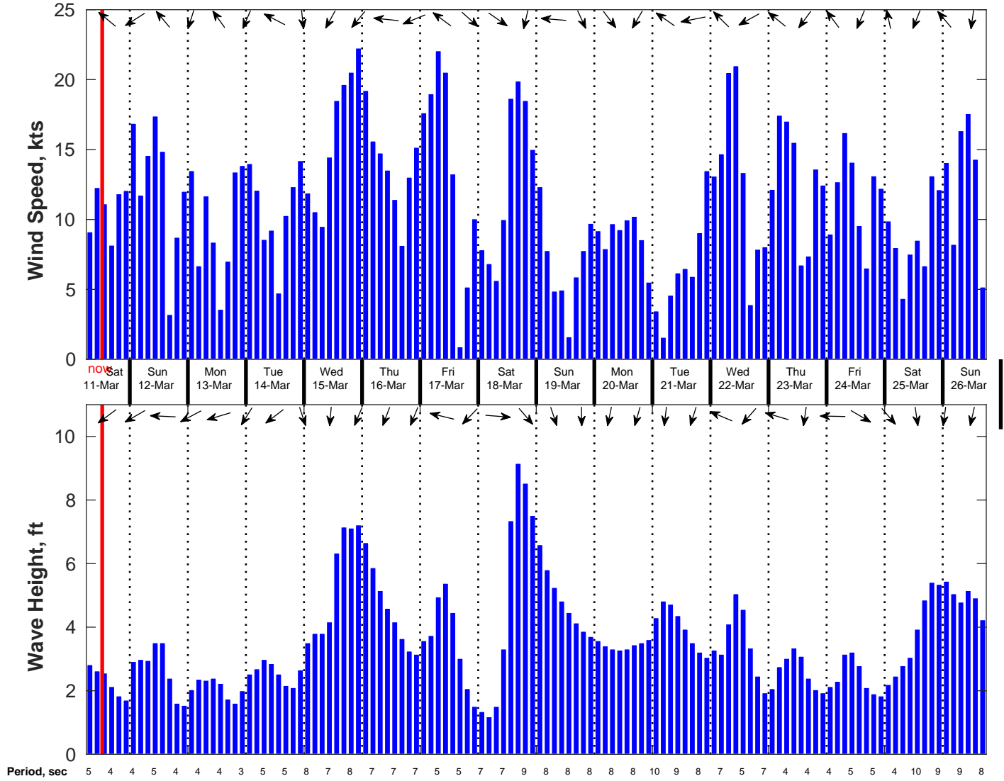
Wind & Wave Forecast for Drebbel MX GT - Natalie from 11-Mar-2023 06:00:00 to 27-Mar-2023 06:00:00
