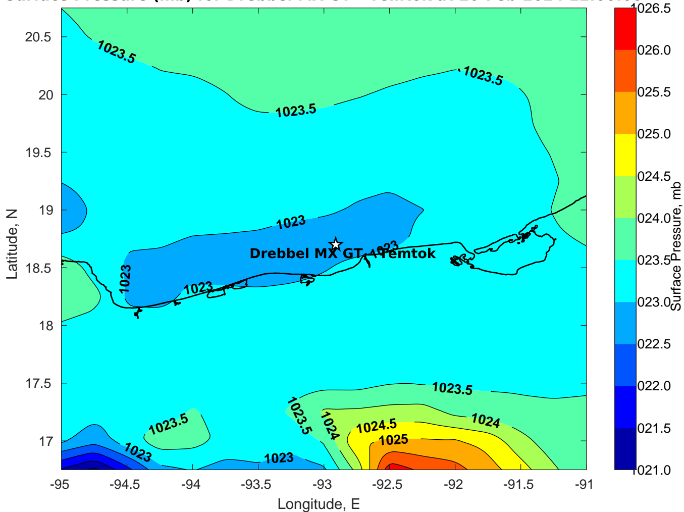
Surface Pressure (mb) for Drebbel MX GT - Temtok at 20-Feb-2024 12:00:00
