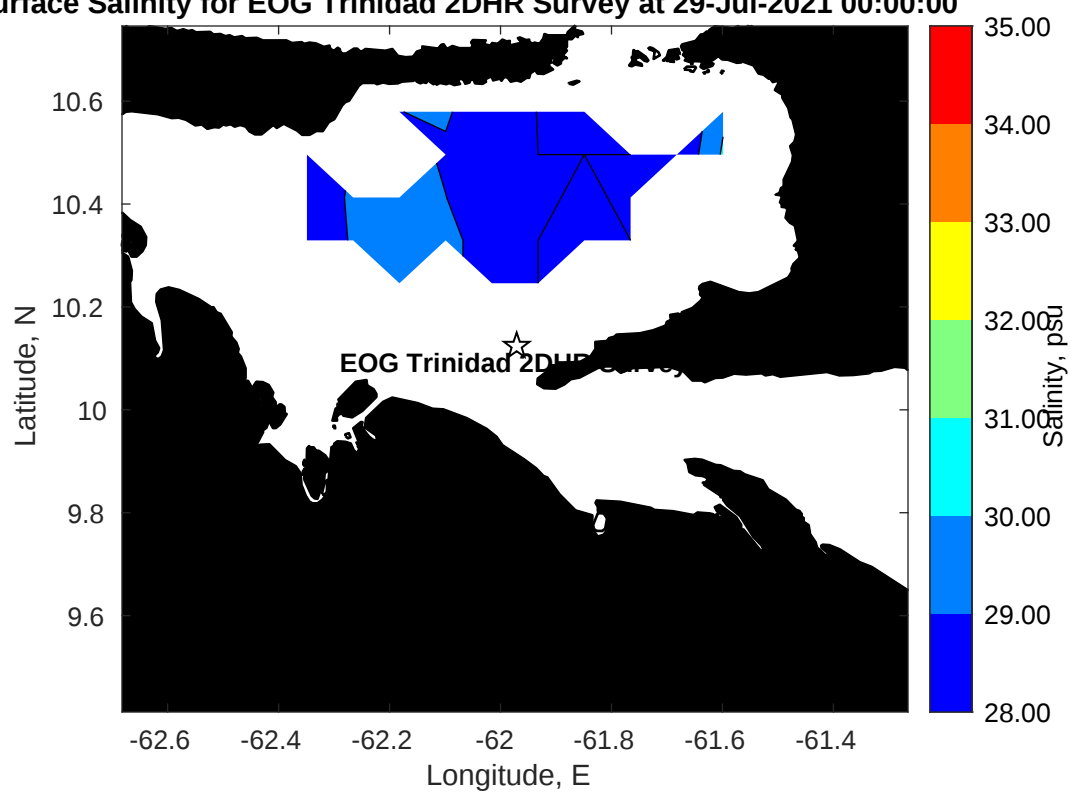
Surface Salinity for EOG Trinidad 2DHR Survey at 29-Jul-2021 00:00:00
