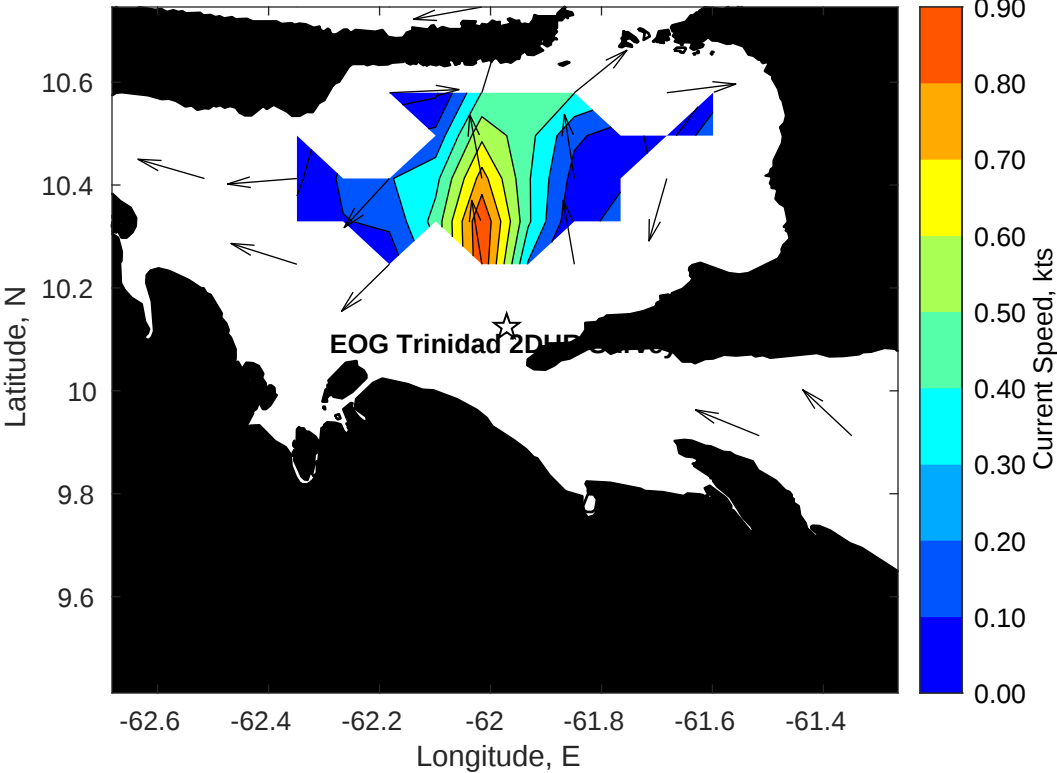
Surface Currents for EOG Trinidad 2DHR Survey at 29-Jul-2021 00:00:00
