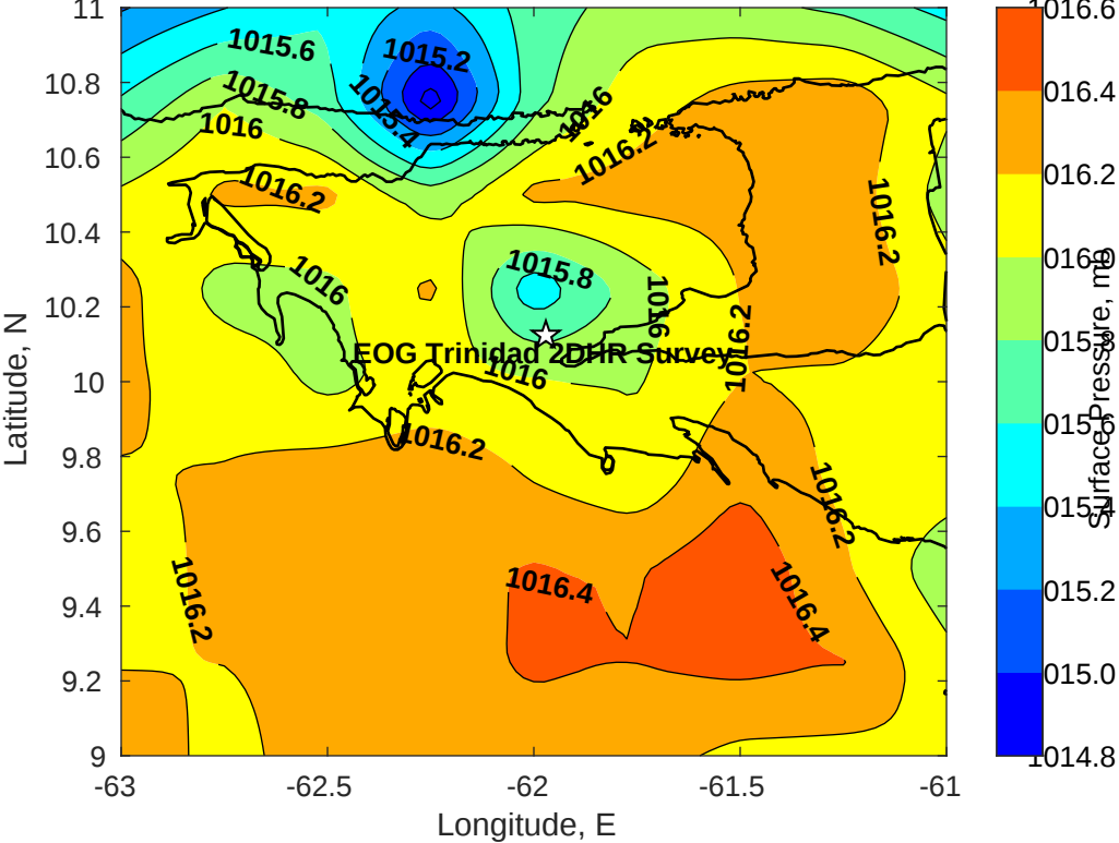
Surface Pressure (mb) for EOG Trinidad 2DHR Survey at 29-Jul-2021 12:00:00
