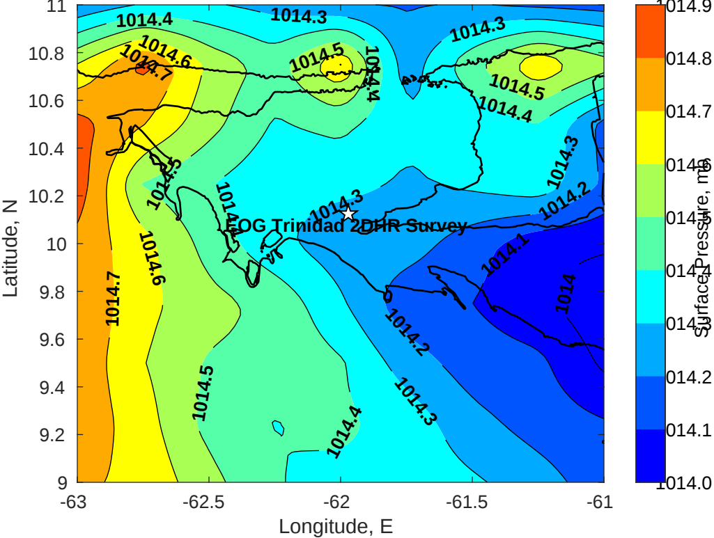
Surface Pressure (mb) for EOG Trinidad 2DHR Survey at 30-Jul-2021 09:00:00
