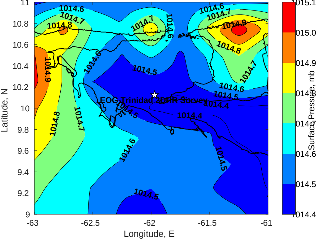
Surface Pressure (mb) for EOG Trinidad 2DHR Survey at 31-Jul-2021 09:00:00
