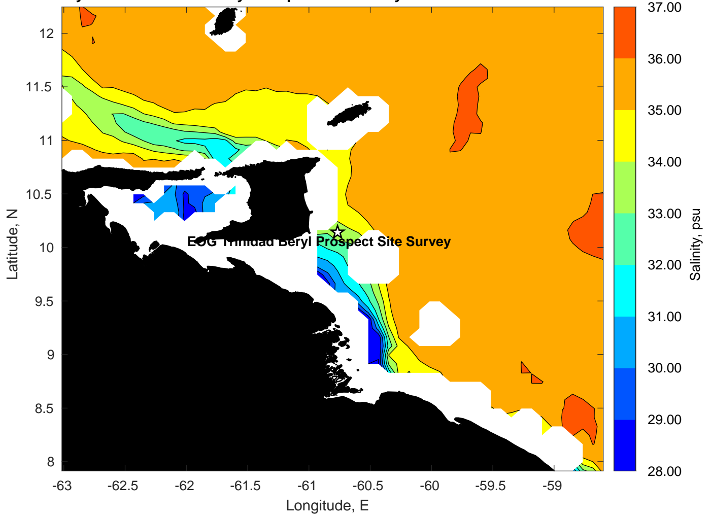
Surface Salinity for EOG Trinidad Beryl Prospect Site Survey at 25-Dec-2023 00:00:00
