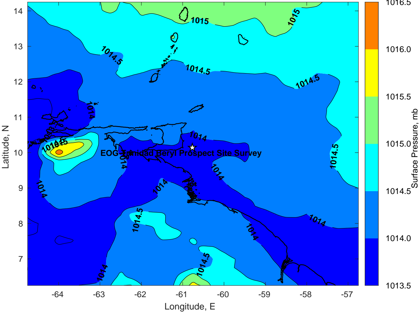
Surface Pressure (mb) for EOG Trinidad Beryl Prospect Site Survey at 25-Dec-2023 12:00:00
