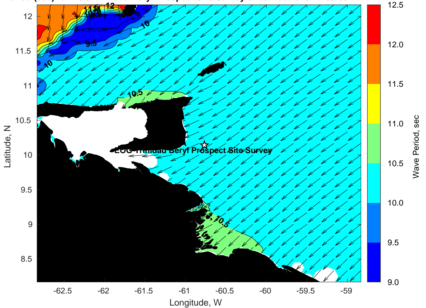
Wave Period (sec) for EOG Trinidad Beryl Prospect Site Survey at 25-Dec-2023 12:00:00
