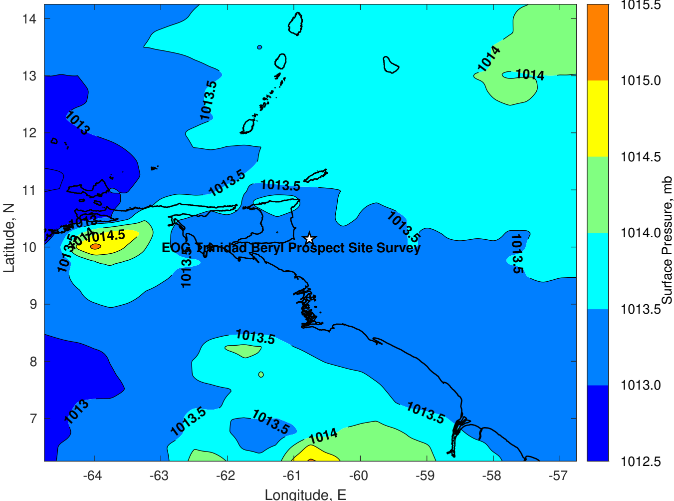
Surface Pressure (mb) for EOG Trinidad Beryl Prospect Site Survey at 27-Dec-2023 12:00:00
