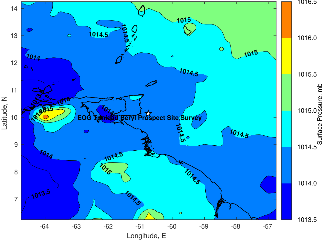
Surface Pressure (mb) for EOG Trinidad Beryl Prospect Site Survey at 26-Dec-2023 12:00:00
