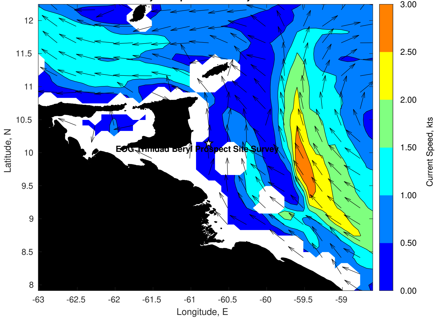
Surface Currents for EOG Trinidad Beryl Prospect Site Survey at 25-Dec-2023 00:00:00
