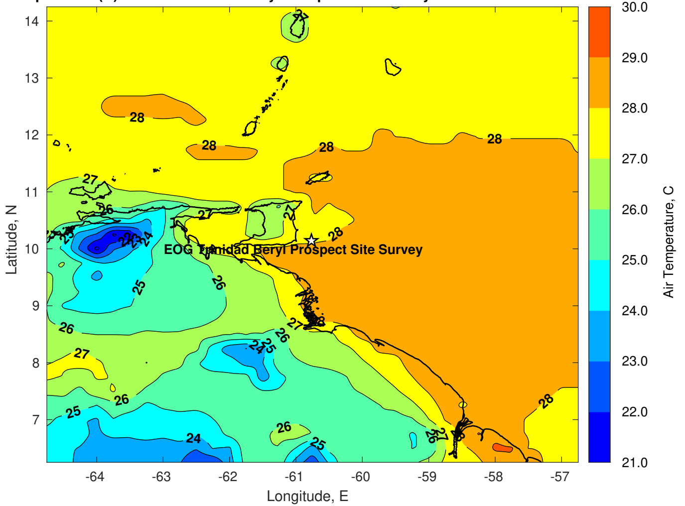
Air Temperature (C) for EOG Trinidad Beryl Prospect Site Survey at 25-Dec-2023
