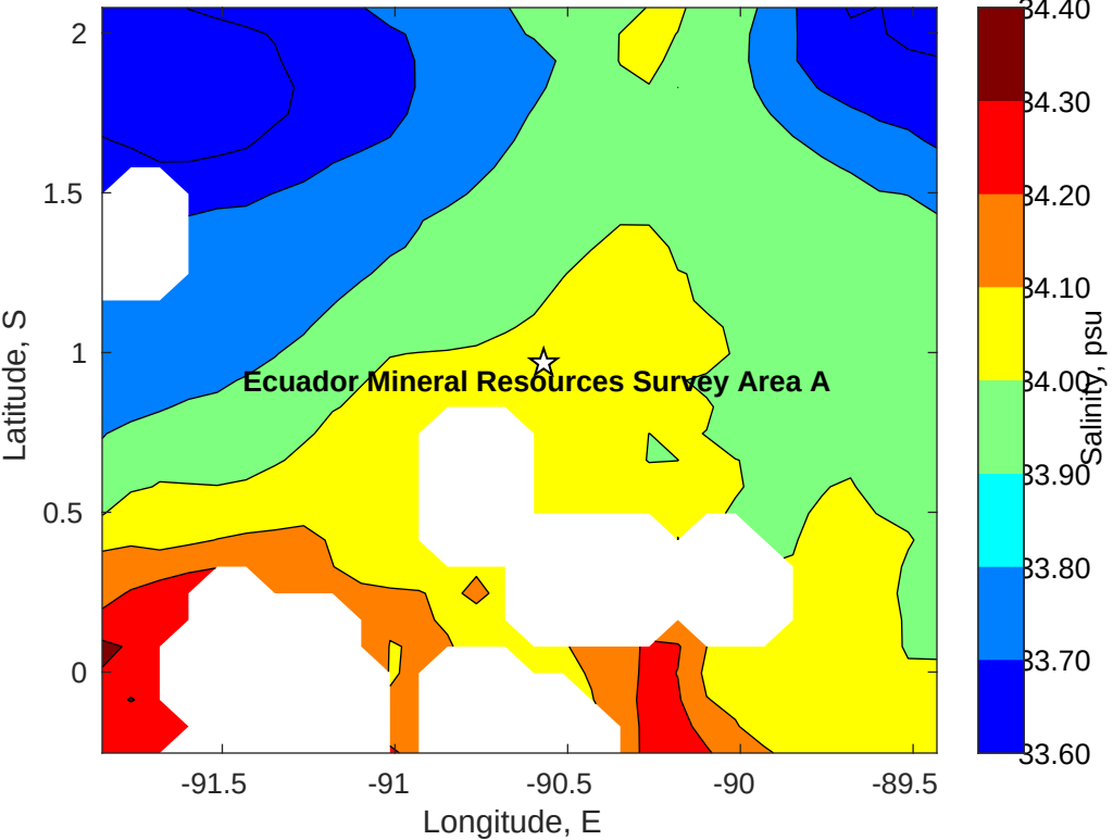
Surface Salinity for Ecuador Mineral Resources Survey Area A at 11-Oct-2021 00:00:00
