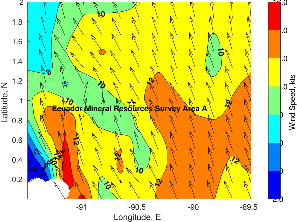
Winds (kts) for Ecuador Mineral Resources Survey Area A at 11-Oct-2021 12:00:00
