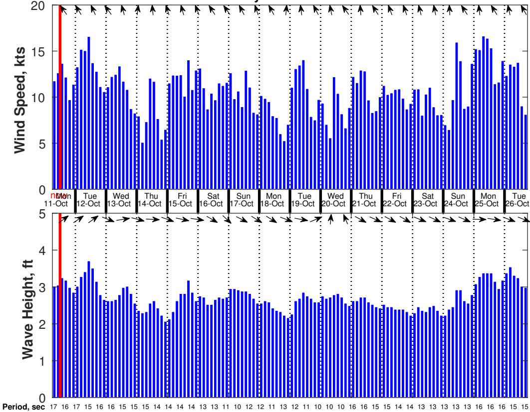
Wind & Wave Forecast for Ecuador Mineral Resources Survey Area A from 11-Oct-2021 06:00:00 to 27-Oct-2021 03:00:00
