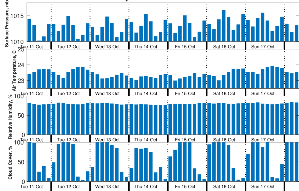
Met Forecast for Ecuador Mineral Resources Survey Area A from 11-Oct-2021 12:00:00 to 18-Oct-2021 12:00:00
