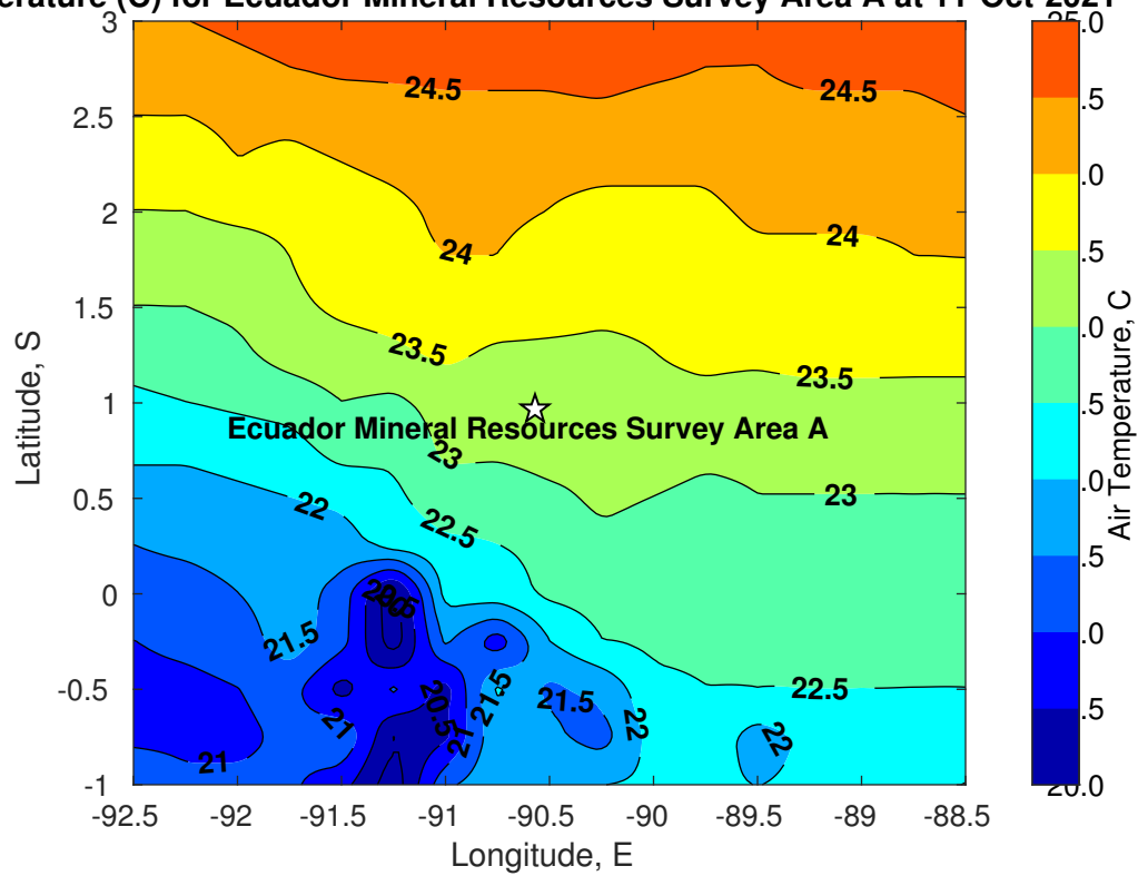
Air Temperature (C) for Ecuador Mineral Resources Survey Area A at 11-Oct-2021
