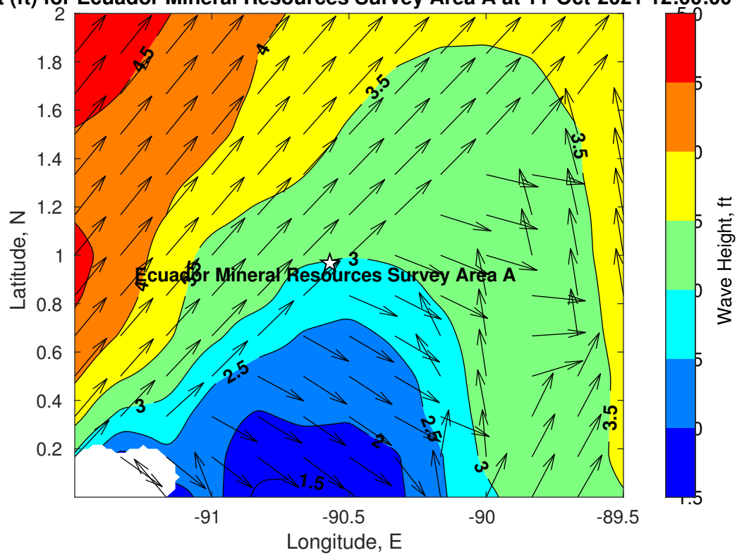
Wave Height (ft) for Ecuador Mineral Resources Survey Area A at 11-Oct-2021 12:00:00
