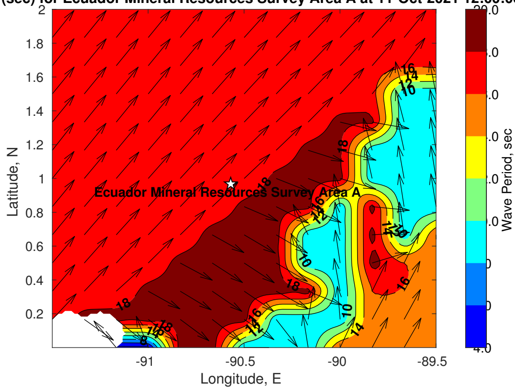
Wave Period (sec) for Ecuador Mineral Resources Survey Area A at 11-Oct-2021 12:00:00
