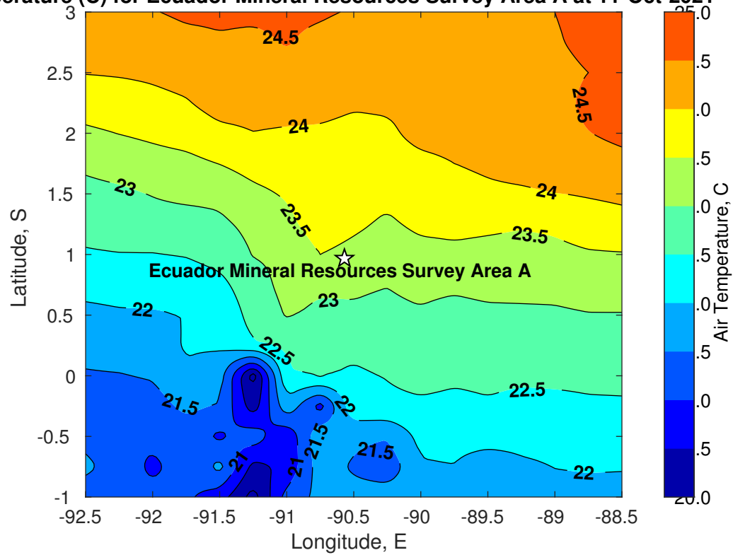
Air Temperature (C) for Ecuador Mineral Resources Survey Area A at 11-Oct-2021
