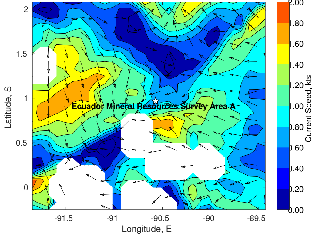
Surface Currents for Ecuador Mineral Resources Survey Area A at 11-Oct-2021 00:00:00
