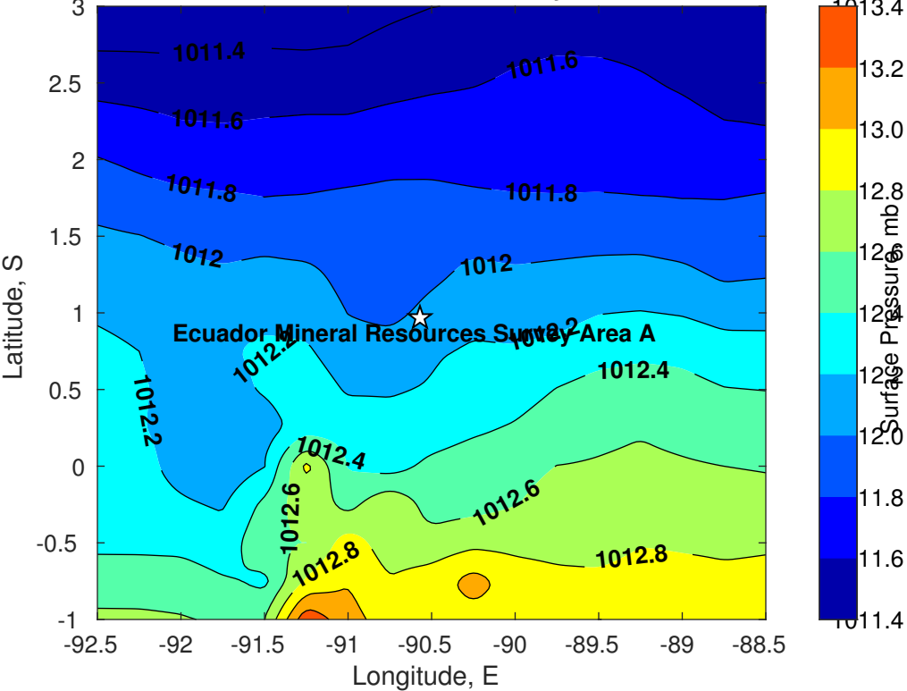
Surface Pressure (mb) for Ecuador Mineral Resources Survey Area A at 12-Oct-2021 09:00:00
