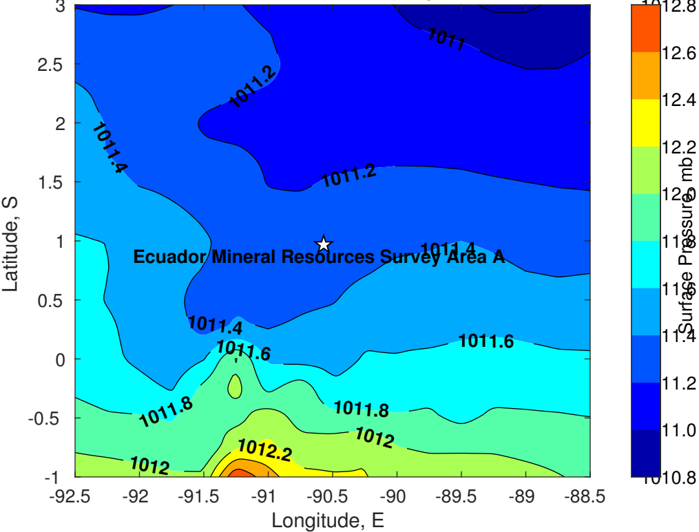
Surface Pressure (mb) for Ecuador Mineral Resources Survey Area A at 13-Oct-2021 09:00:00
