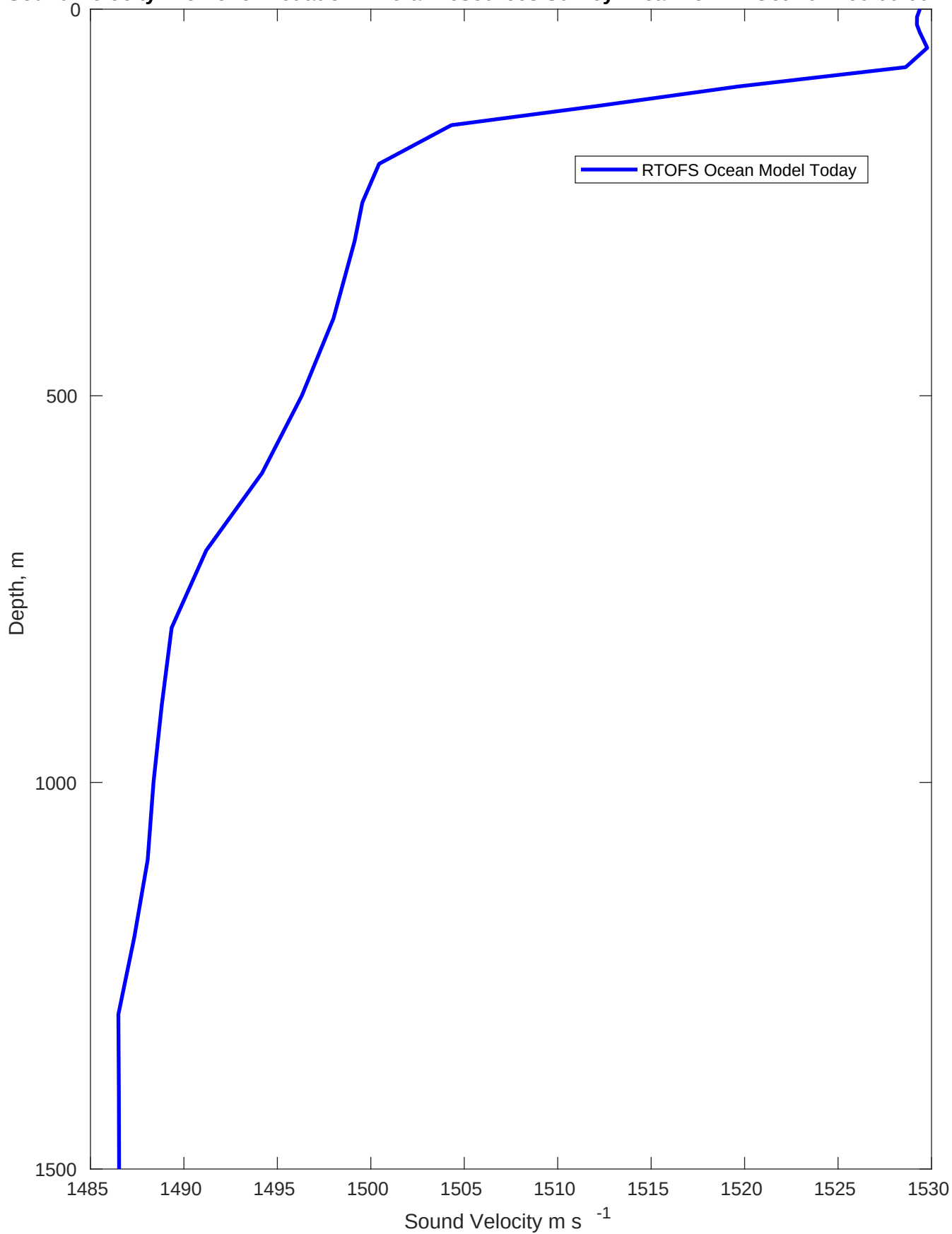
Sound Velocity Profile for Ecuador Mineral Resources Survey Area A on 11-Oct-2021 00:00:00
