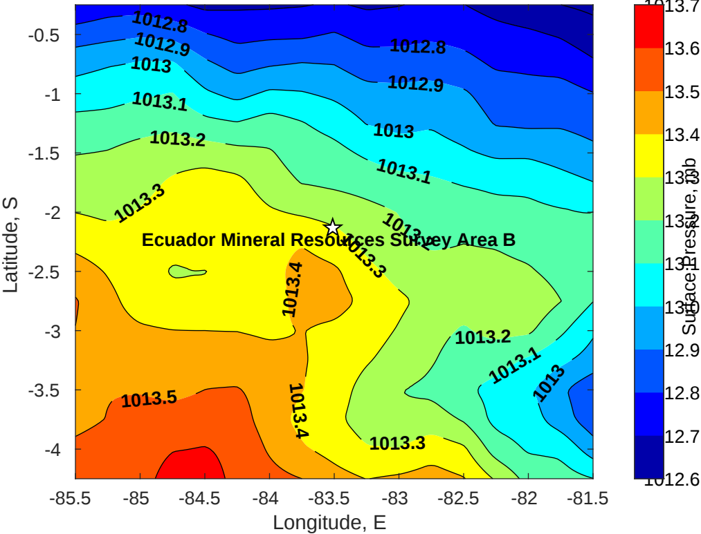
Surface Pressure (mb) for Ecuador Mineral Resources Survey Area B at 11-Oct-2021 12:00:00
