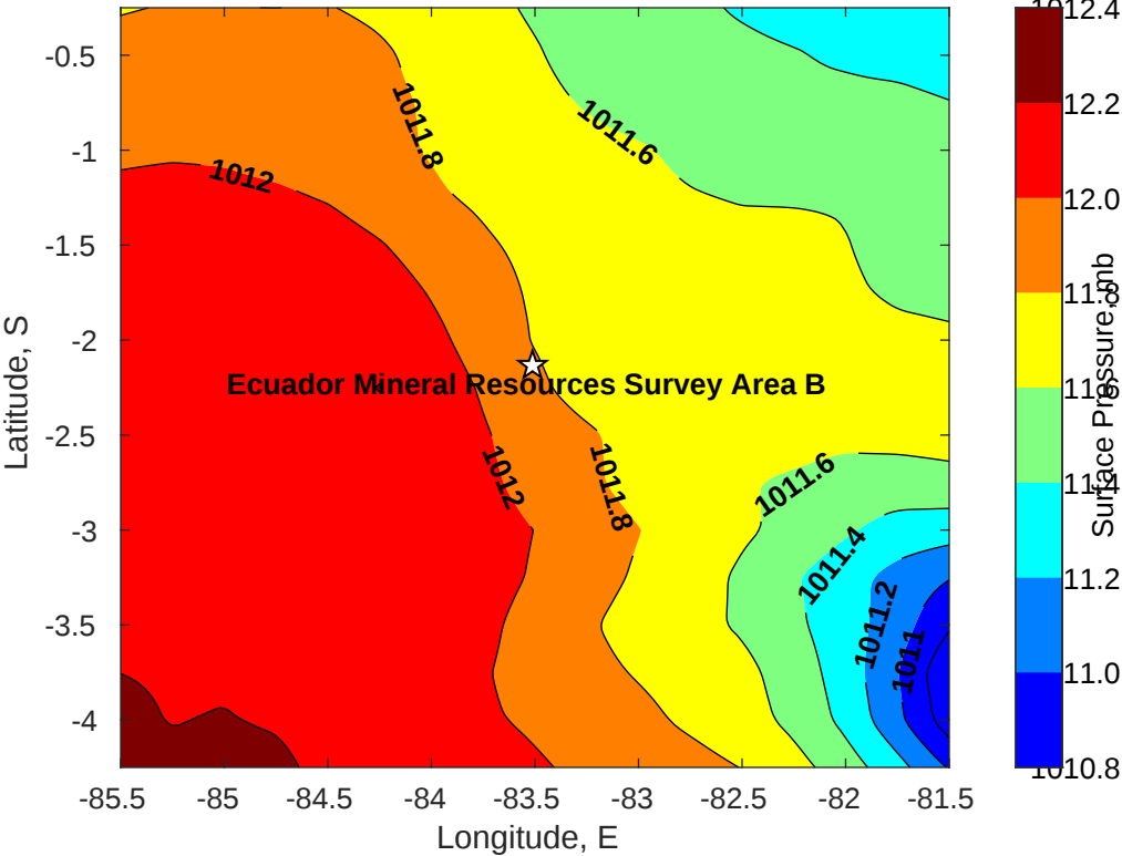
Surface Pressure (mb) for Ecuador Mineral Resources Survey Area B at 13-Oct-2021 09:00:00
