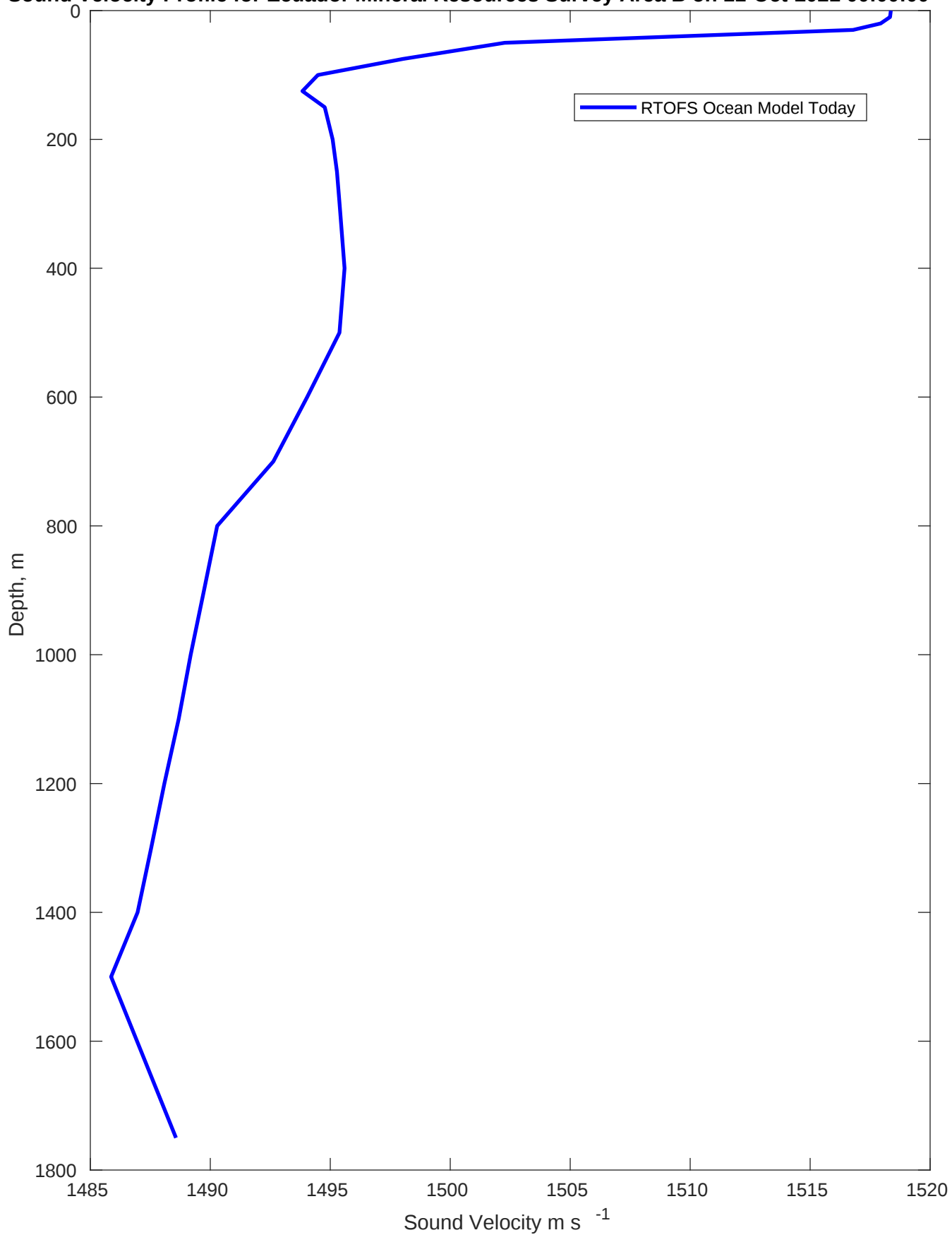
Sound Velocity Profile for Ecuador Mineral Resources Survey Area B on 11-Oct-2021 00:00:00
