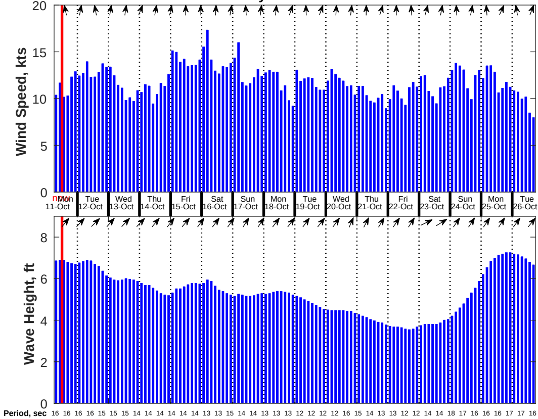
Wind & Wave Forecast for Ecuador Mineral Resources Survey Area B from 11-Oct-2021 06:00:00 to 27-Oct-2021 03:00:00
